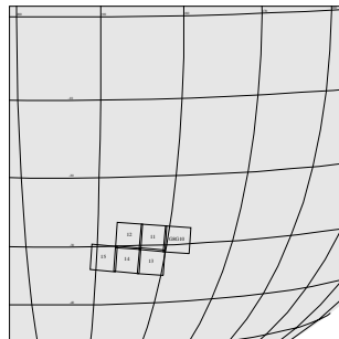
G8GSCALDRA01 GTE-CDS 39:00:0 97-127/15:16:45
