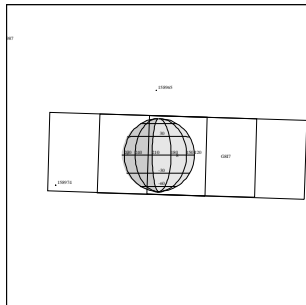
G8ISAMRANI01 IEE-CDS 86:00:0 97-127/06:03:40
