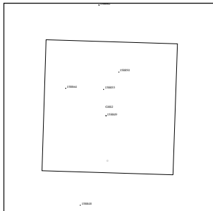
G8SSADRAST02 JEE-CDS 1954:00:0 97-127/02:46:30
