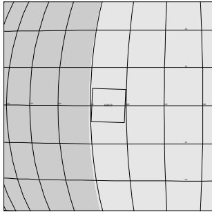
G8STIAMAT01 GTE-CDS 100:60:0 97-127/14:14:24
