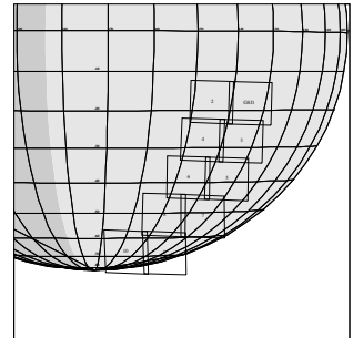
G8JSSOTEMP01 JEE-CDS 1986:00:0 97-127/02:14:09
