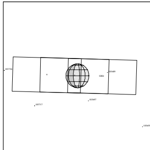
G8ISKANEHI01 IEE-CDS 514:00:0 97-126/22:50:55
