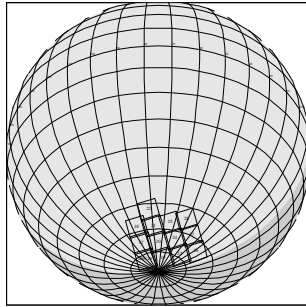
G8CSSPOLAR01 CEE-CDS 5:00:0 97-126/12:05:50
