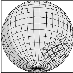
G8CSVGRGAP01 CEE-CDS 76:00:0 97-126/10:54:02
