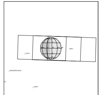
G8ISPROMTH01 IEE+CDS 184:00:0 97-127/10:36:40
