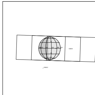
G8ISMALIK_01 IEE+CDS 20:00:0 97-127/07:50:51
