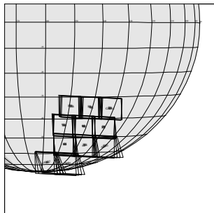
G8JSSOTEMP03 JEE-CDS 1390:00:0 97-127/12:16:46
