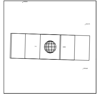
G8ISECLIPS01 IEE-CDS 923:00:0 97-126/15:57:22
