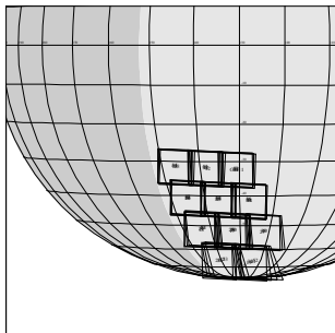
G8JSSOTEMP02 JEE-CDS 1449:00:0 97-127/11:17:07
