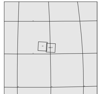
G8GSANSHAR01 GTE-CDS 34:00:0 97-127/15:21:48
