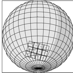
G8CSADLND01 CEE+CDS 56:00:0 97-126/13:07:30
