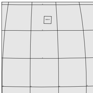
G8GSPITCRA01 GTE-CDS 33:00:0 97-127/15:22:49
