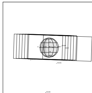
G8ISMARDUK01 IEE+CDS 658:00:0 97-127/18:35:56
