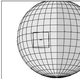
G8CSPHOTOM01 CEE+CDS 234:00:0 97-126/16:07:29
