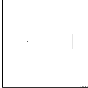
C3SSTHEBE_01 IEE-CDS 21:00:0 96-311/11:43:34
