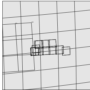
C3CSVALGRB01 CTE+CDS 4:70:0 96-309/13:38:57
