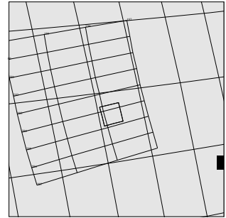
C3CSVALPLM01 CTE-CDS 1:00:0 96-309/13:33:07
