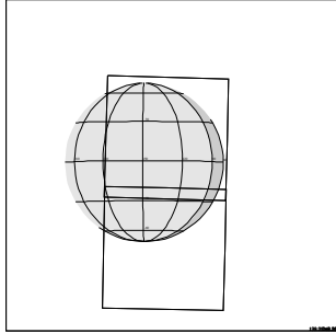
C3ISTOPMAP01 IEE-CDS 356:00:0 96-311/06:04:50
