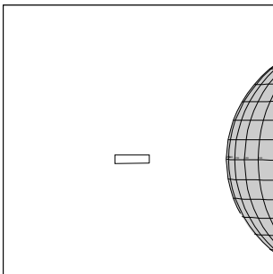
C3RSRINGS_02 JOC+CDS 63:00:0 96-314/07:12:03
