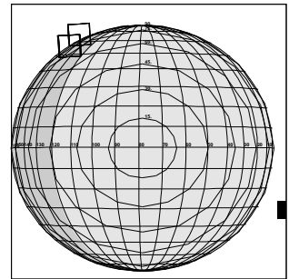
C3JSAURRGN02 JTB-CDS 161:00:0 96-310/05:12:27
