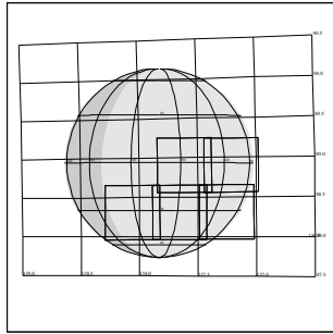
C3CSVGRGAP01 CEE-CDS 364:00:0 96-309/07:22:03
