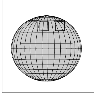
C3JSLTGSCN01 JOC-CDS 67:00:0 96-314/05:00:36
