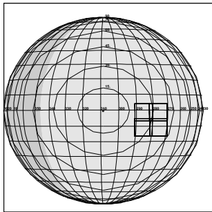
C3JSBZONEB01 JTA-CDS 568:00:0 96-310/01:30:00
