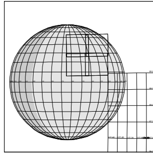
C3CSASGRNG01 CEE-CDS 244:00:0 96-309/09:23:23
