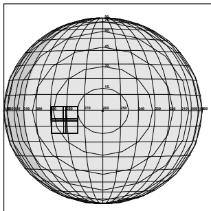
C3JSBZONEB02 JTA-CDS 40:00:0 96-310/10:23:52
