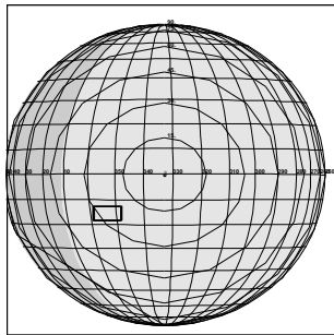
C3JSHICOLR01 JTA-CDS 527:00:0 96-310/02:11:27
