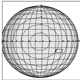
C3JSHICOLR02 JTA-CDS 442:00:0 96-310/03:37:24
