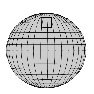
C3JSLTGSP01 JOC-CDS 84:39:0 96-314/04:42:59
