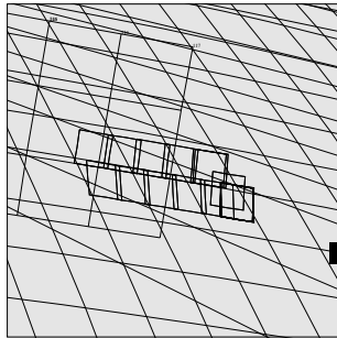
C3CSVALPLN01 CTE+CDS 3:70:0 96-309/13:37:57
