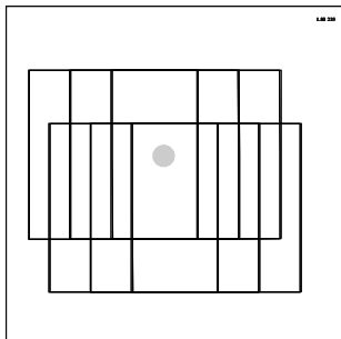
C3ESPLUMES01 JOC-CDS 88:00:0 96-314/04:39:22
