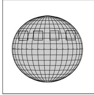
C3JSLTGSCN02 JOC-CDS 63:45:0 96-314/05:04:09
