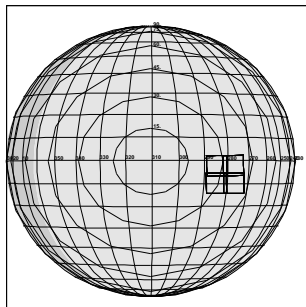
C3JSBZONEB03 JTA+CDS 47:00:0 96-310/11:51:50
