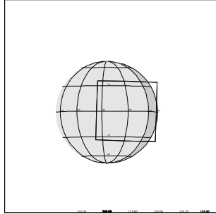
C3ISTOPMAP02 IEE-CDS 148:00:0 96-311/09:35:09
