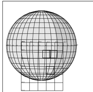
C3ESWEDGES01 EEE+CDS 56:00:0 96-311/19:46:52
