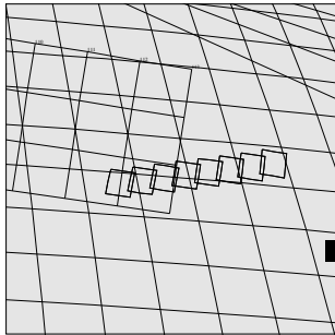
C3CSCATENA01 CTE+CDS 1:45:0 96-309/13:35:39
