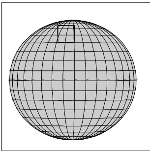
C3JSAURORA04 JOC+CDS 45:00:0 96-314/06:53:51
