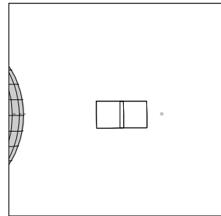
C3RSGOSSMR01 JOC+CDS 59:00:0 96-314/07:08:00
