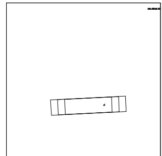
C3ASAMLTHE01 IEE-CDS 979:00:0 96-310/19:34:55
