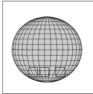
C3JSLTGSCN06 JOC-CDS 45:00:0 96-314/05:22:51
