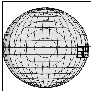
C3JSBZONEB04 JTA+CDS 107:00:0 96-310/12:52:30
