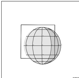
C3ISTOPMAP05 IEE+CDS 476:00:0 96-311/20:06:05
