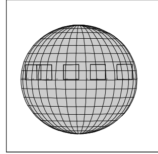
C3JSLTGSCN03 JOC-CDS 59:45:0 96-314/05:08:12
