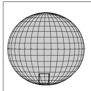
C3JSAURORA02 JOC-CDS 76:00:0 96-314/04:51:30
