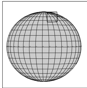
C3JSAURORA06 JOC+CDS 55:00:0 96-314/07:03:58
