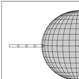
C3RSRINGS_01 JOC-CDS 115:00:0 96-314/04:12:04
