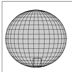
C3JSAURORA01 JOC-CDS 80:00:0 96-314/04:47:28
