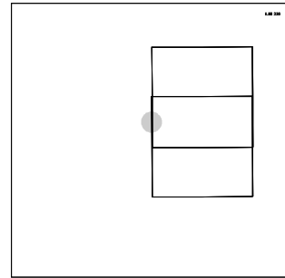
C3ISNA_CLD01 JOC-CDS 41:00:0 96-314/05:26:54
