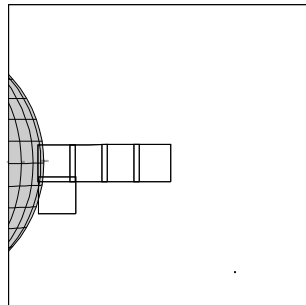
C3RSRNGHAL01 JOC-CDS 97:00:0 96-314/04:30:16
