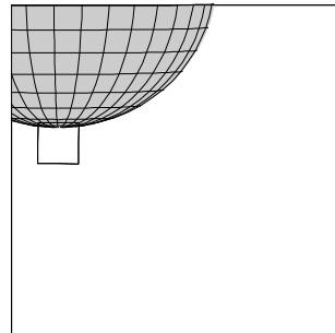
C3JSLIMBHZ01 JOC-CDS 92:00:0 96-314/04:35:20
