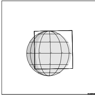
C3CSHEMCLR01 CEE-CDS 1054:00:0 96-308/19:44:23
