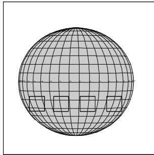
C3JSLTGSCN05 JOC-CDS 49:45:0 96-314/05:18:18
