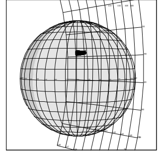
C3CNARINGS01 CTE-CDS 42:00:0 96-309/12:51:40
