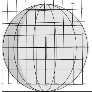
C3CNCALLRT02 CEE-CDS 247:00:0 96-309/09:20:21
