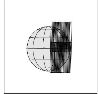
C3INTHRMAL01 96-311/12:24:00
