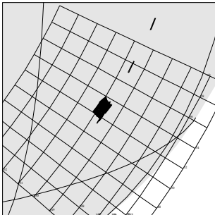
C3CNCRATER01 CTE-CDS 13:00:0 96-309/13:20:59
