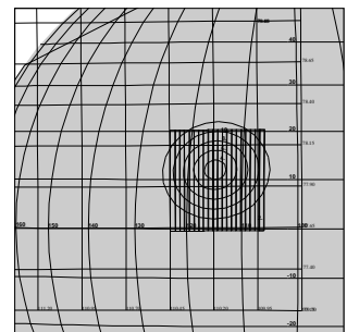
C3JNOCSPEC01 96-314/05:52:10
