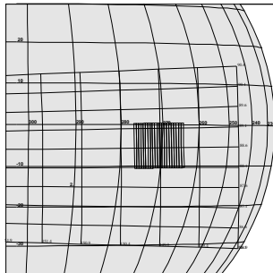
C3JNFEASUB01 JTA+CDS 34:00:0 96-310/11:38:41
