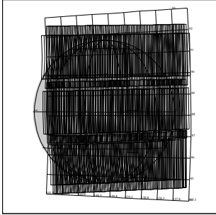
C3CNGLOBAL01 CEE-CDS 444:00:0 96-309/06:01:09
