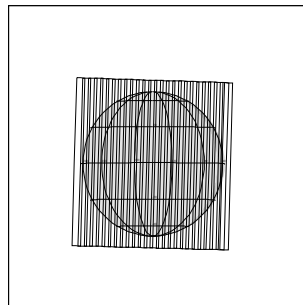
C3INCHEMIS02 96-311/04:00:28
