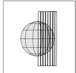
C3INTHRMAL03 96-311/23:45:30
