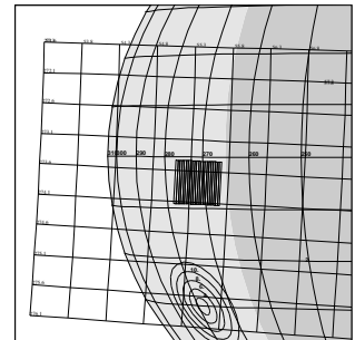
C3JNFEA13603 96-312/05:53:33
