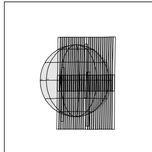
C3INTHRMAL02 96-311/15:12:52
