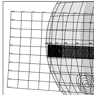
C3JNFEA13601 96-312/05:23:13
