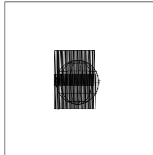
C3INCHEMIS04 96-311/16:00:23
