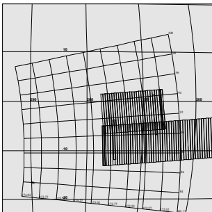
C3JNFEA01104 JTA+CDS 630:00:0 96-310/21:41:19
