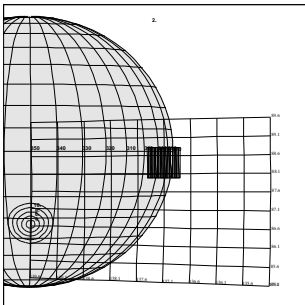
C3JNFEA05103 JTA-CDS 495:00:0 96-310/02:43:49
