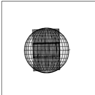
C3ENPHINEA01 96-311/14:24:17
