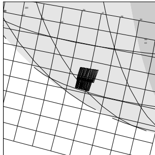
C3CNCSPOTS01 CTE+CDS 17:00:0 96-309/13:51:19
