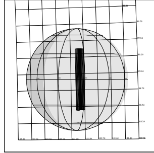
C3ENEURORT01 96-311/09:53:37
