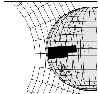
C3JNFEA01101 JTC+CDS 511:00:0 96-310/19:40:59
