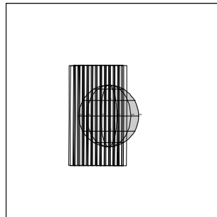
C3INCHEMIS05 96-312/00:03:42
