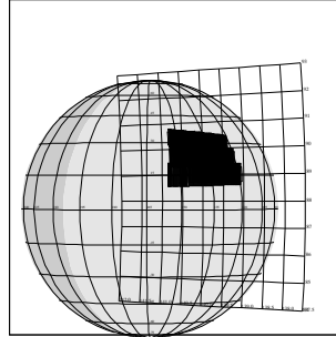
C3CNASGARD01 CTE-CDS 90:00:0 96-309/12:03:08
