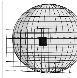
C3JNFEA05101 JTA-CDS 644:00:0 96-310/00:13:09
