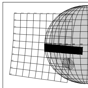
C3JNFEA15301 96-312/15:38:59
