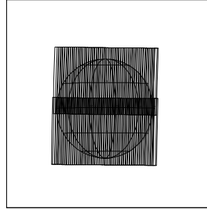
C3INHRSPEC01 96-311/11:48:37
