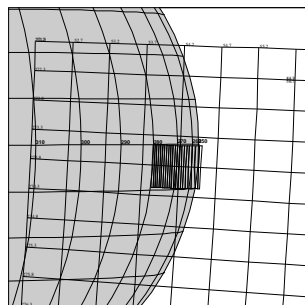
C3JNFEA5UM02 96-312/09:01:37
