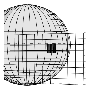
C3JNFEA05102 JTA-CDS 574:00:0 96-310/01:23:56
