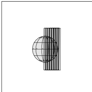
C3INVOLCAN01 96-311/23:57:38
