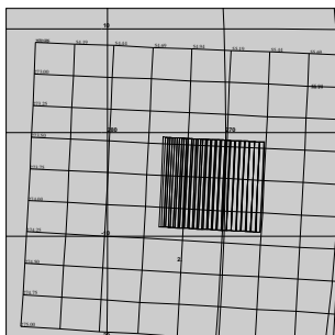
C3JNFEA53M01 96-312/07:26:34
