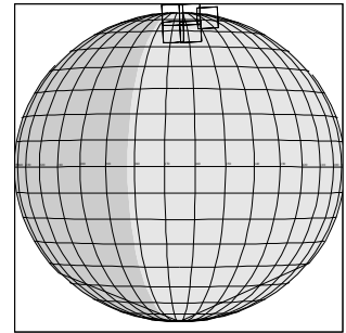
10JSNPHAZE03 JEE-CDS 1245:00:0 97-261/02:11:25
