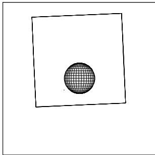
10ISIOECLI01 IEE-CDS 1498:00:0 97-261/03:29:17
