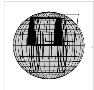
10JSLIGHTN02 97-278/22:22:44
