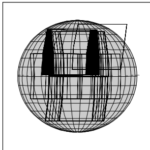
10JSLIGHTN03 97-278/22:58:07
