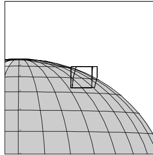
10JSFLXTUB01 97-262/23:24:14
