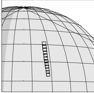
10CSASGARD01 CTE-CDS 26:00:0 97-259/23:53:05
