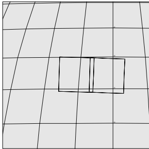
10CSRNGSTR01 CTE+CDS 45:00:0 97-260/01:04:52
