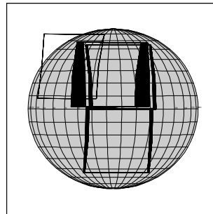
10JSLIGHTN04 97-279/00:13:57
