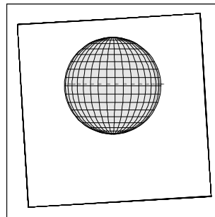
10ESGLOBAL01 EEE+CDS 428:00:0 97-262/12:33:05
