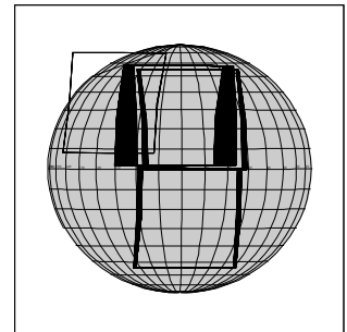
10JSLIGHTN05 97-279/01:28:47
