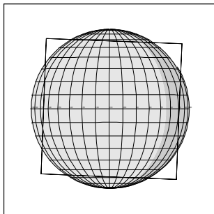
10ISIOTOPO02 IEE-CDS 368:00:0 97-261/22:31:50
