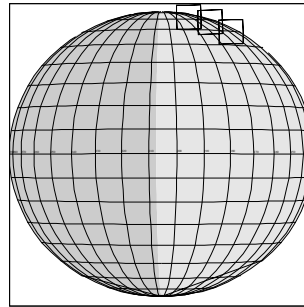
10JSNPHAZE02 JEE-CDS 1793:00:0 97-260/16:57:20
