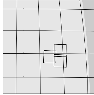
10CSSMTHPL02 CTE+CDS 29:00:0 97-260/00:48:42
