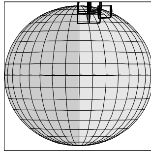
10JSNPHAZE01 JEE-CDS 1853:00:0 97-260/15:56:40
