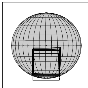
10JSAURORA01 97-279/02:06:11
