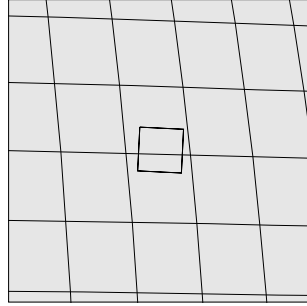
10CSSMTHPL01 CTE+CDS 15:00:0 97-260/00:34:32
