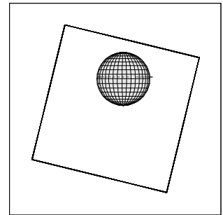
10GSGLOCOL01 GEE-CDS 54:00:0 97-261/17:02:13
