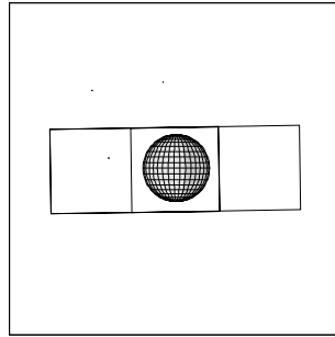
10ISIOECLI02 97-262/22:01:19
