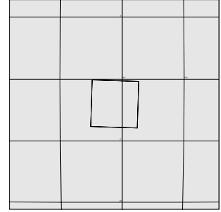
10CSTINDR_01 CTE+CDS 43:00:0 97-260/01:02:51
