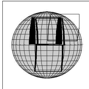
10JSLIGHTN01 97-278/21:19:02
