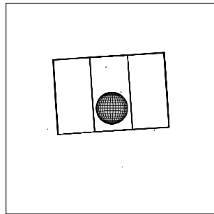
10ISIOGLOC01 IEE-CDS 1256:00:0 97-261/07:33:05
