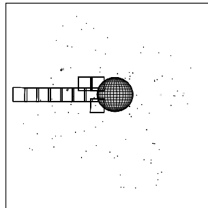
10RSRINGS_01 97-278/23:53:44
