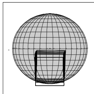
10JSAURORA02 97-279/02:16:18
