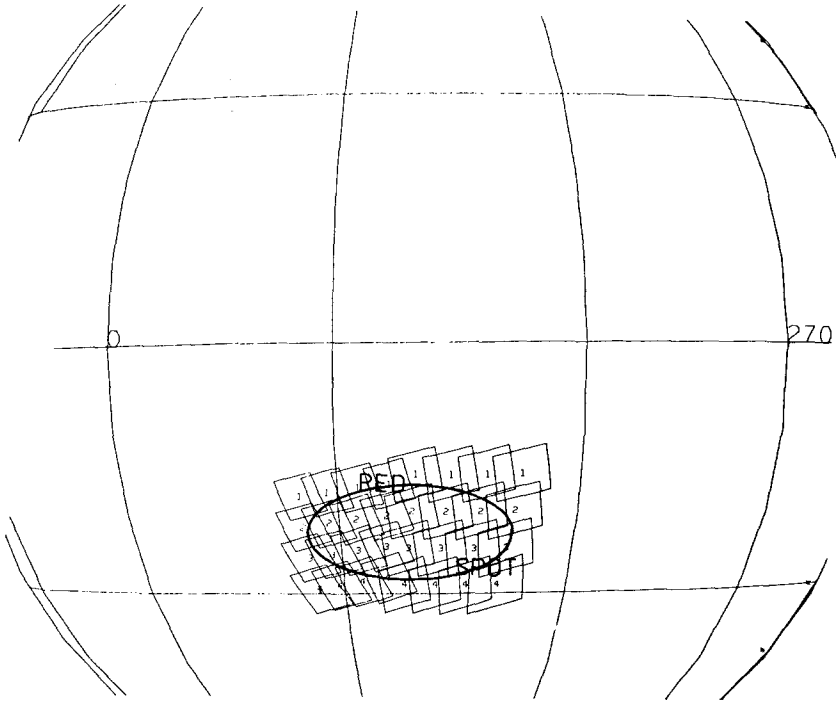
Fig. 13. Two color mosaic of the Great Red Spot. Several Great Red Spot observations will be made on approach to Jupiter. Shown is an ISSNA two-color mosaic planned to be taken on the JST Trajectory about 8 hours before Jupiter closest approach.
