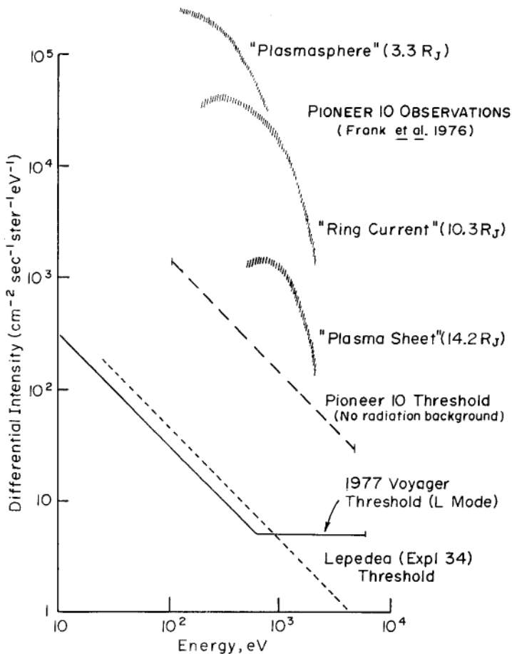
Fig. 8. The predicted sensitivity of the Voyager instrument in the Jovian environment compared with the sensitivity of some other instruments using intensities expected on the basis of the Pioneer 10 results.
