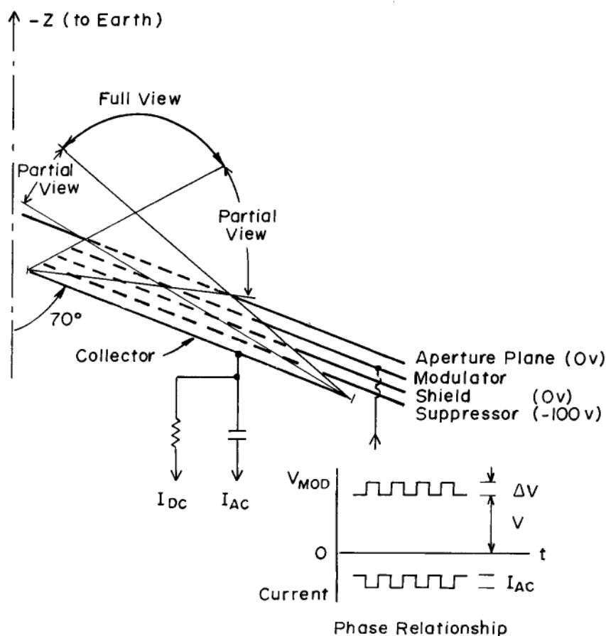
Fig. 2. A cross sectional view of the grid structure (schematic) for one of the three sensors of the -Z detector. For clarity only a single shield grid and a single modulator grid are shown. In the actual sensor six shield grids are used to obtain sufficient electrical isolation between the modulator and collector, and three grids are used for the modulator so that the retarding potential is defined to 0.5%.
