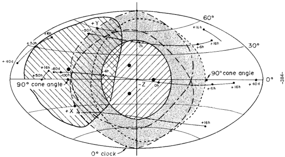
Fig. 3. The fields of view of the four plasma sensors projected onto an all sky map. The origin of the coordinate system is the -Z axis of the spacecraft; the +X and +Y axes are also shown, and the position of 0^\circ 'clock angle' defined by the Canopus star tracker is indicated. The four large dots represent the directions of the normals of the four sensors. The three dots closest to the origin are the three view directions of the -Z detector, and the dashed lines show the limits of the partial view cones of these sensors. Similarly, the solid closed curve to the left of the origin shows the partial view cone for the lateral sensor. The central circular area consists of the three full view cones of the -Z detector; it defines the primary field of view used for solar wind measurements. The dotted area is the secondary field for the -Z detector. In a magnetosheath or magnetosphere the useful field of view is defined by the combined partial view cones for all four sensors.
