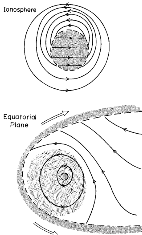
Fig. 7. Magnetospheric flow topology for the corotation-dominated case. (After Vasyliunas, 1975.)
