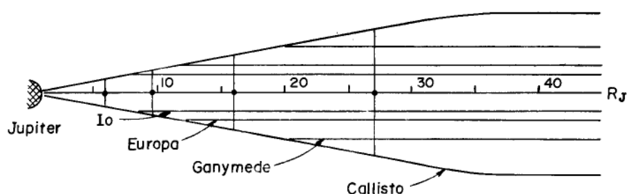
Fig. 9. The ion confinement discs corresponding to each of the Galilean satellites. The horizontal central line is the magnetic equator. The common flaring angle is 10^\circ corresponding to the diurnal excursion of each satellite relative to the magnetic equator. The satellites, dots, and their diurnal excursions are indicated by the labeled vertical lines. The lower limit of the confinement disc of each satellite is also labeled by an arrow from the satellite's name.
