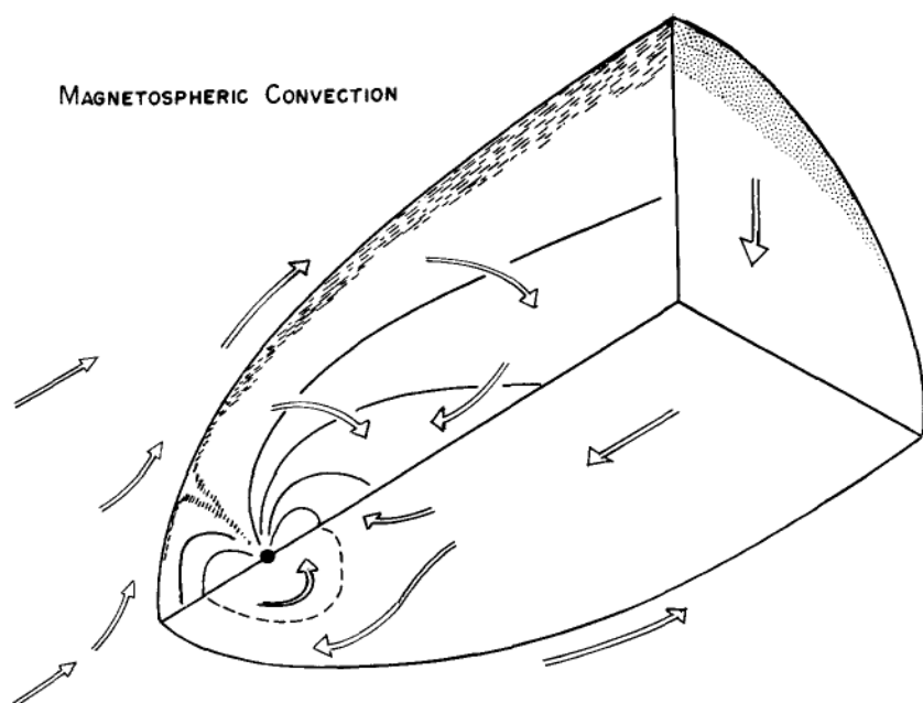
Fig. 5. Circulation patterns of magnetospheric convection in Earth's magnetosphere. The shaded region denotes the boundary layer formed by the entry of external plasma into the magnetosphere. (After Vasyliunas, 1976).
