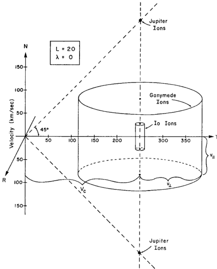
Fig. 10. The regions in velocity space occupied by ions from the neutral particle rings of Io and Ganymede and from Jupiter's ionosphere. The spatial location of the example is at a Jovicentric distance of 20R_J and in the magnetic equatorial plane. The axes are: V_R , the radial (from planet) velocity component; V_T , the velocity component in the direction of corotation; and V_N , the northward velocity component. In this case the V_N direction is parallel to the magnetic field (ignoring the 10^\circ tilt).
