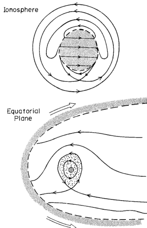
Fig. 6. Magnetospheric flow topology for the convection-dominated case. (After Vasyliunas, 1975.)
