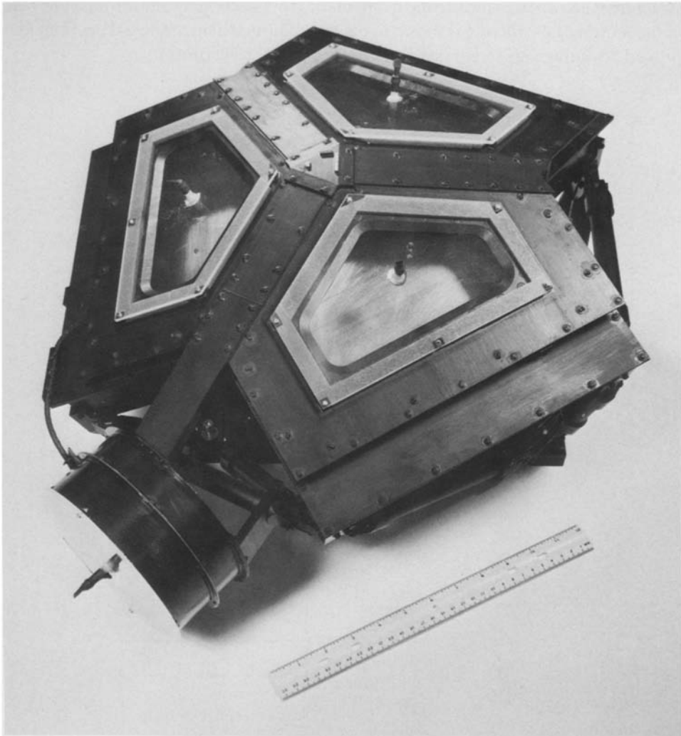
Fig. 1. Photograph of the Voyager plasma instrument. The three apertures of the main sensor are visible; the lateral detector is in the lower left region of the view. The axis of symmetry of the main sensor cluster is directed parallel to the -Z axis of the spacecraft (the Earth-pointing direction). In this photograph the apertures of the sensors are closed by protective covers which are removed before launch; each cover is fitted with a connection for a purge gas.
