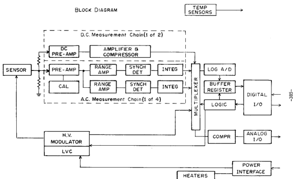
Fig. 4. Block diagram of the Voyager plasma instrument for one of the four sensors. The dc measurement chains measure the total positive or negative currents to the collector of one sensor in the -Z detector and to the collector of the lateral detector.
