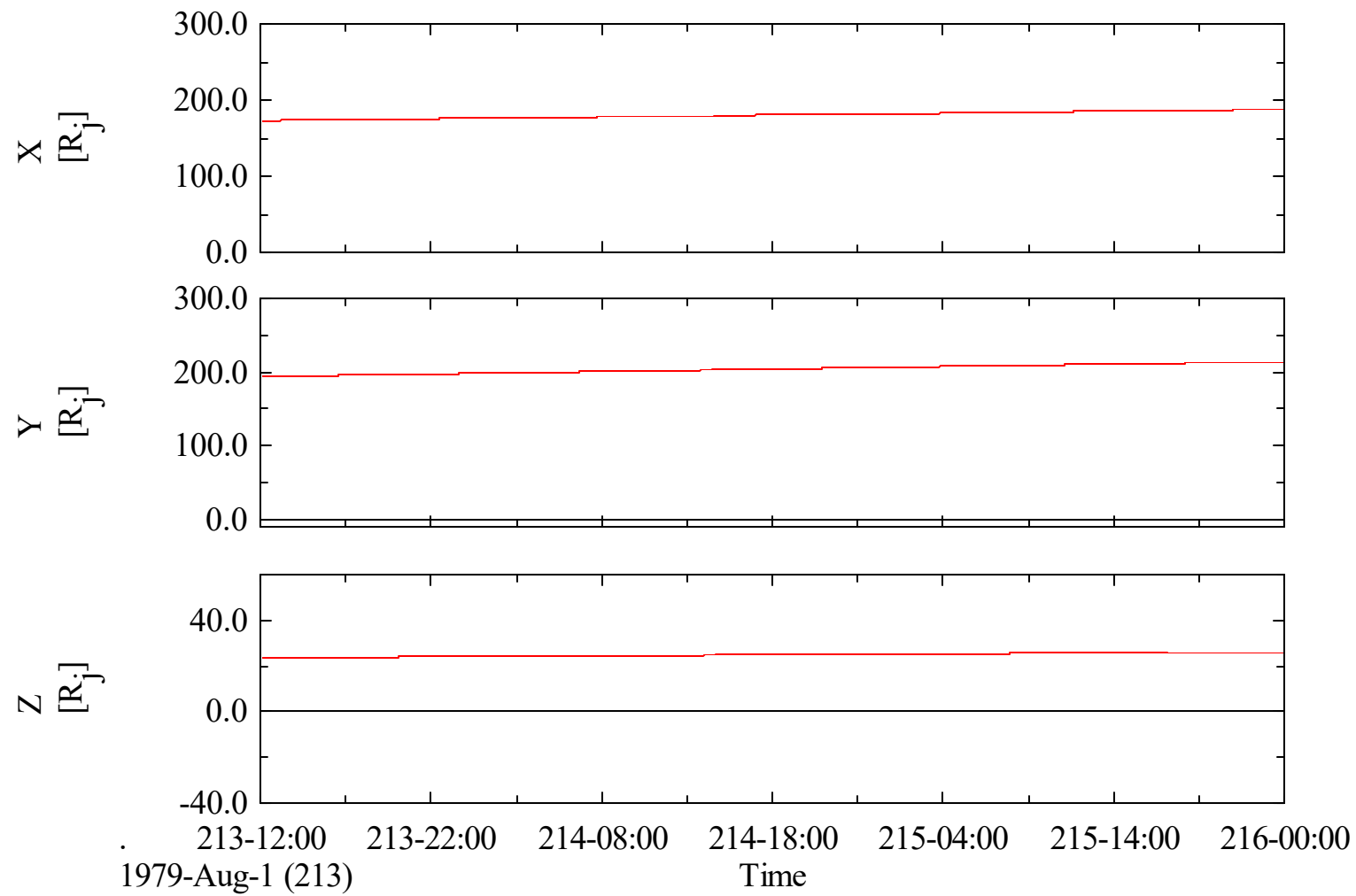
Voyager 2 EPHEM 96 Second Data in System III (1965) at Jupiter
