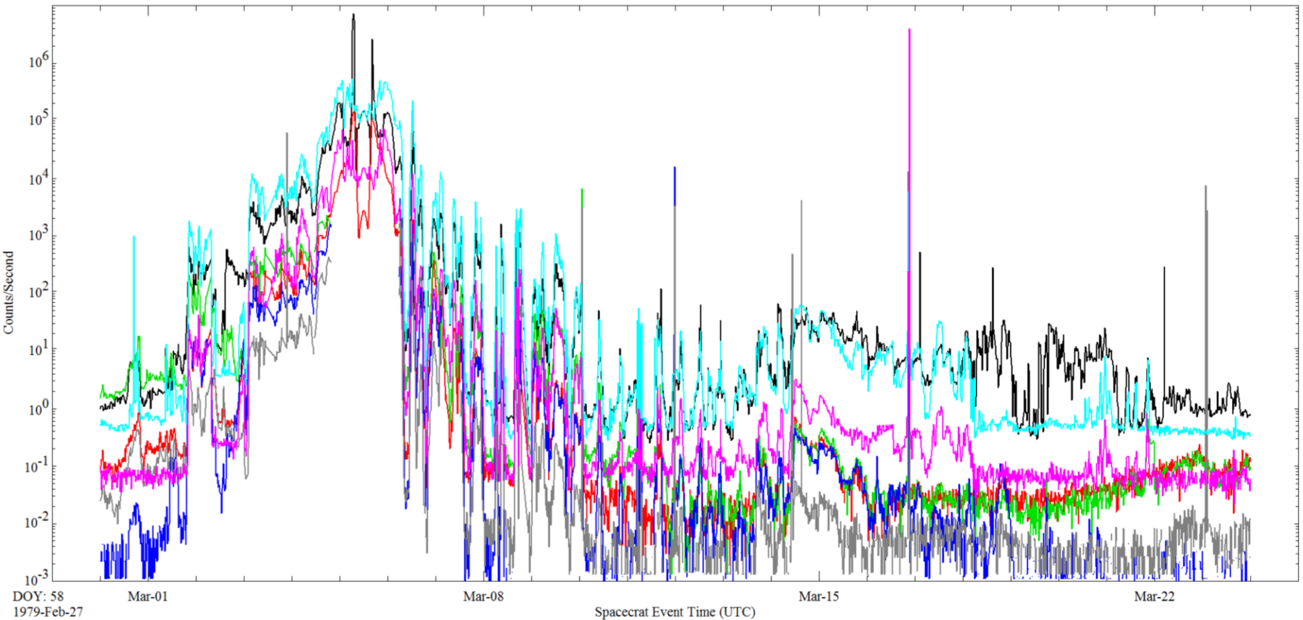
Voyager 1 LECP Charged Particle Counting Rate at Jupiter
