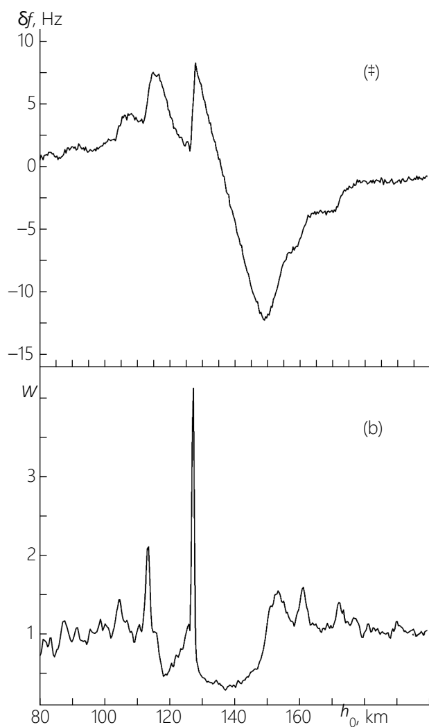
Fig. 2. (a) Reduced frequency \delta f and (b) power W of a decimeter-wavelength signal as functions of altitude h_0 . The results are obtained from the data of the radio exit of October 22, 1983. ( z \approx 68.8^\circ ).
