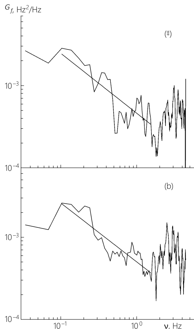
Fig. 6. Spectra G_f(\nu) of frequency fluctuations: (a) the radio exit of October 22, 1983, z = 69^\circ , and the altitudes 250–430 km and (b) the radio exit of October 25, 1983, z = 73.5^\circ , and the altitudes 300–480 km. The straight lines show the power dependence.
