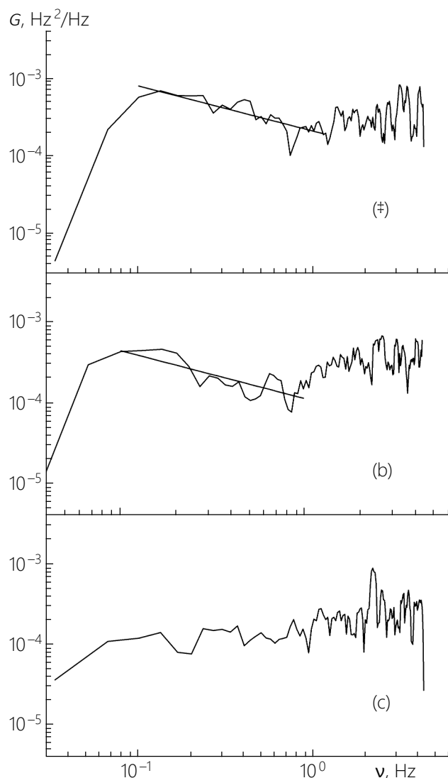
Fig. 5. Spectra G_f(\nu) of frequency fluctuations for three altitude intervals: (a) 250–357 km, (b) 400–501 km, and (c) 700–782 km. The results are obtained for the radio entry of October 14, 1983, and z = 82^\circ . The straight lines show the power dependence.
