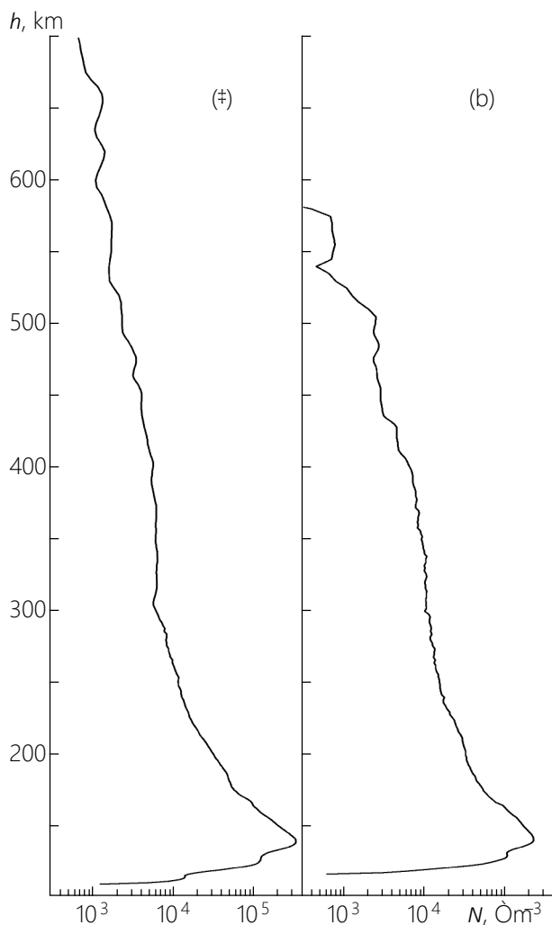
Fig. 4. Altitude distributions N(h) of the electron concentration in the Venusian daytime ionosphere: (a) the radio exit of October 22, 1983, z = 69^\circ and (b) the radio entry of October 14, 1983, z = 82^\circ .
