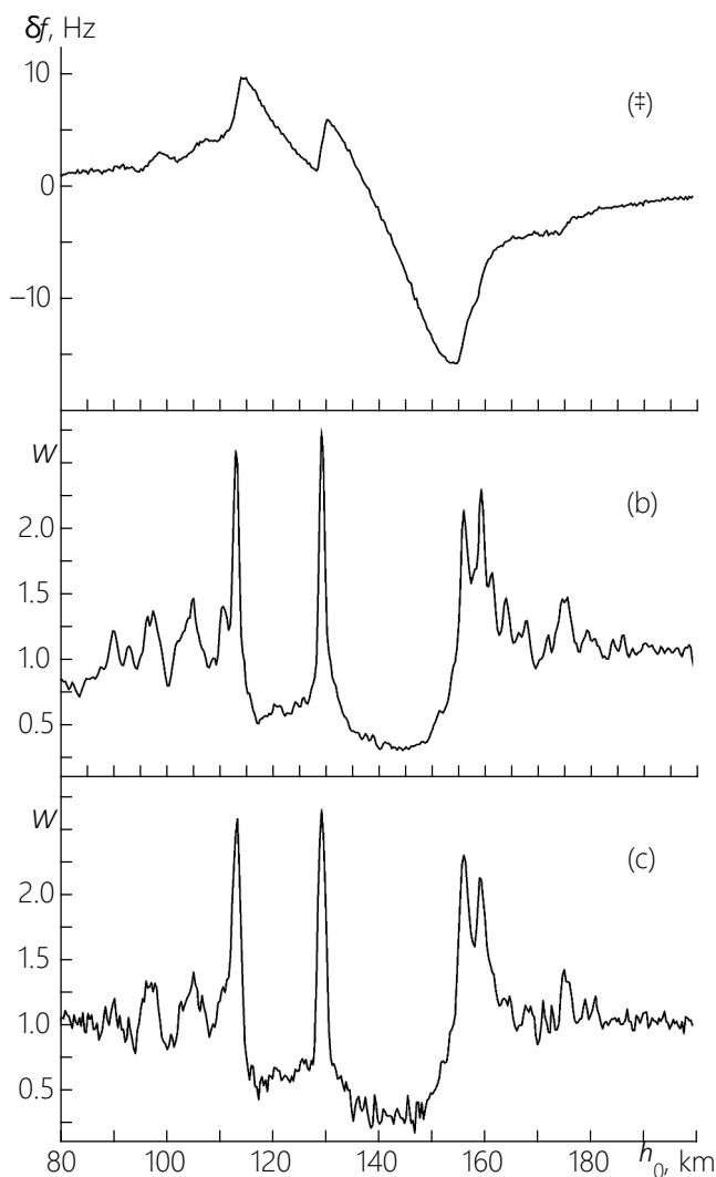
Fig. 1. (a) Reduced frequency \delta f and (b) power W of a decimeter-wavelength signal as functions of altitude h_0 (for the radio exit of October 14, 1983) and (c) the change of the power determined from frequency measurements.
