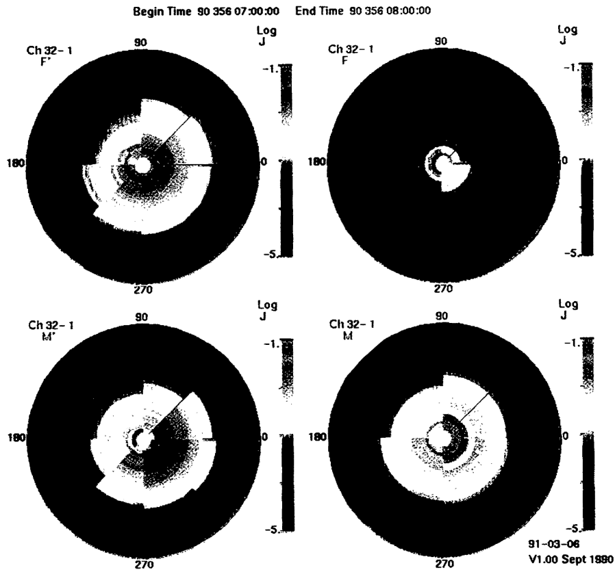
FIGURE 14. Ion spectra plotted as function of angular distribution to illustrate the angular sectoring of the HI-SCALE instrument. The intense low energy fluxes in the M detector are due to sunlight.
