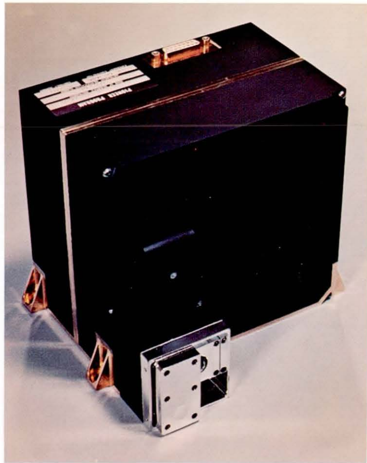
Figure 4-6. Other telescopes are used to explore the radiation belts of Jupiter, measuring electrons and protons in these belts.
