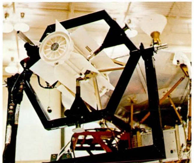
Figure 3-5. Two RTGs are mounted at the end of each of two extended booms to reduce nuclear radiation effects on the sensitive scientific instruments.
