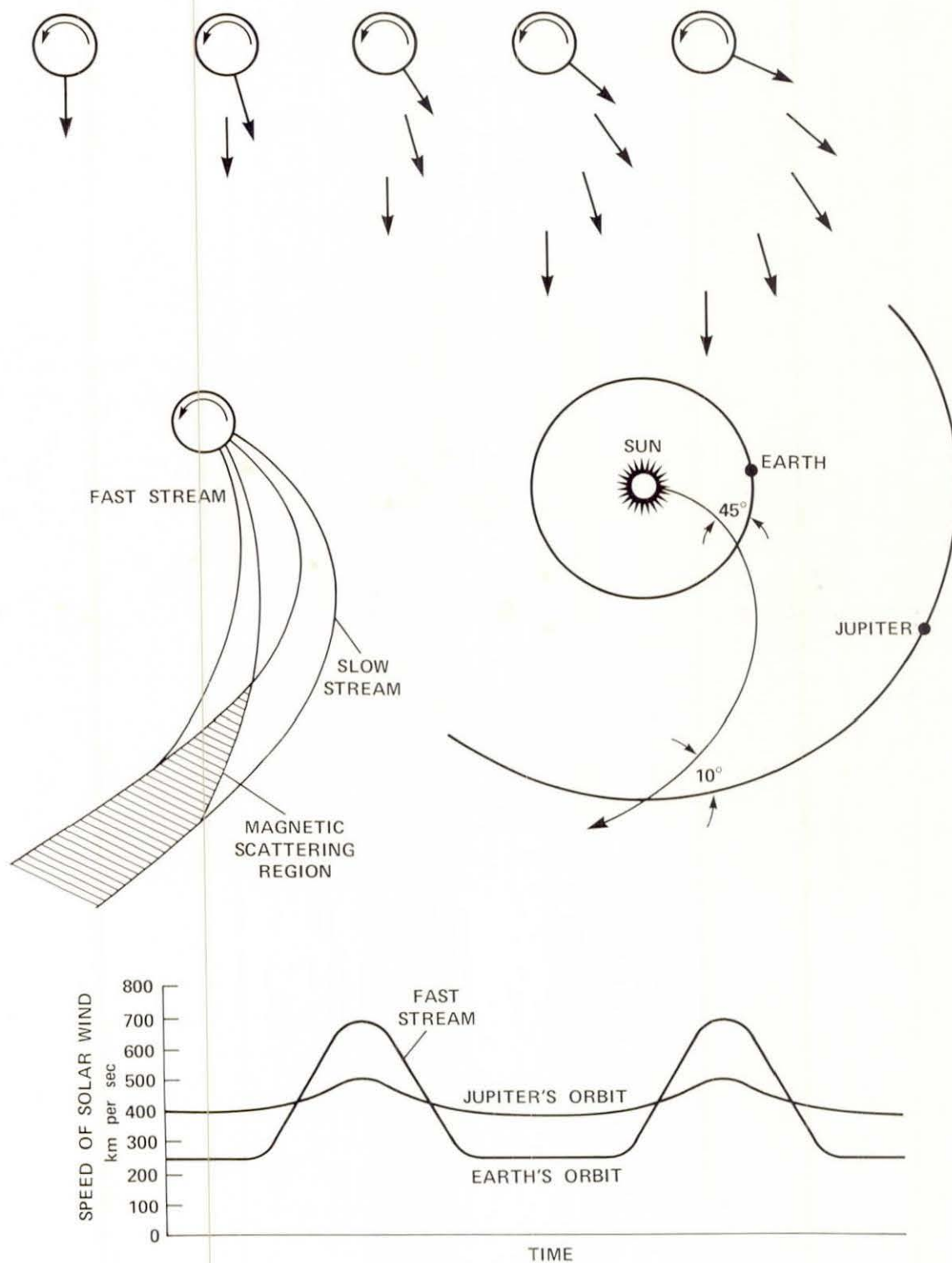
Figure 6-1. Fast streams of solar wind catch up with slow streams and produce scattering regions that prevent low energy cosmic rays from penetrating into the Solar System. Pioneer 10 may reach the boundary where this scattering effect ends.
