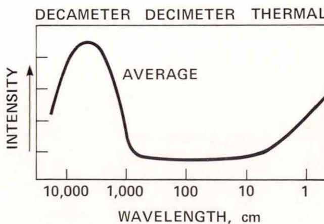
Figure 1-14. Jupiter emits radio waves which have been recorded and measured by radio astronomers for several decades. They are of three main types: thermal, decimetric and decametric. Each has a different origin.
