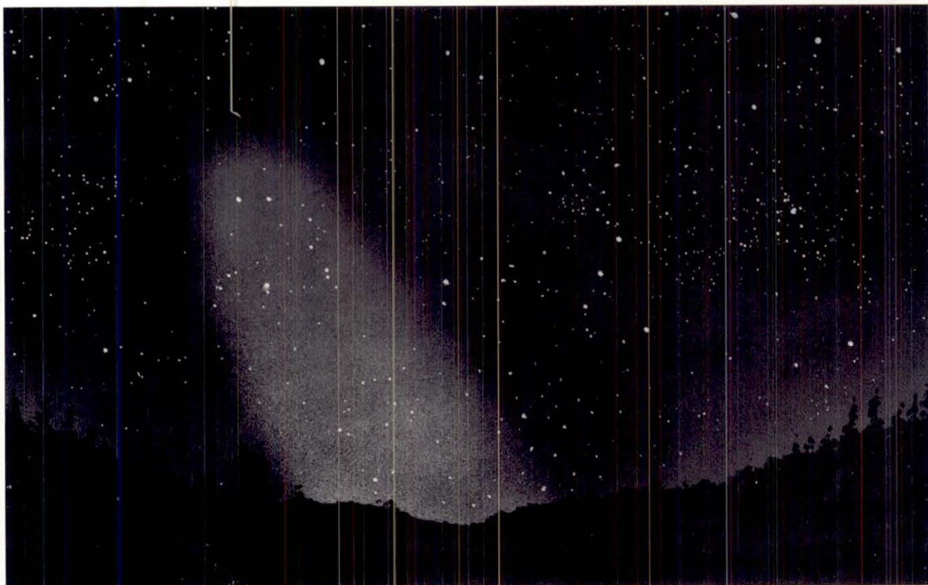
Figure 5-5. A first task was to investigate the Zodiacal Light, a faint glow seen in dark Earth skies after sunset and before sunrise.
