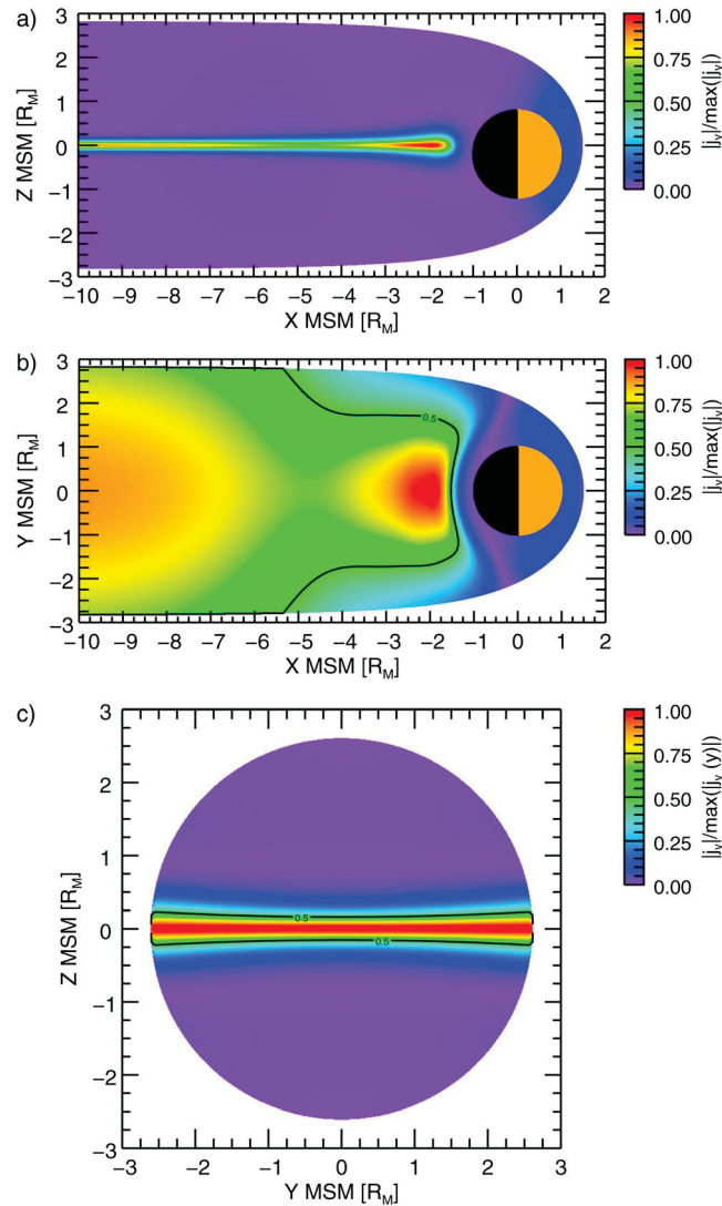
Figure 4. Distribution of dawn-to-dusk current density in the MSM (a) x-z plane at y = 0 R_M , (b) x-y plane at z = 0 R_M , and (c) y-z plane at x = -2 R_M . Current densities in Figures 4a and 4b are normalized to the maximum value in the respective plane. Current density in Figure 4c is normalized to the maximum value at a given y value in that plane.
