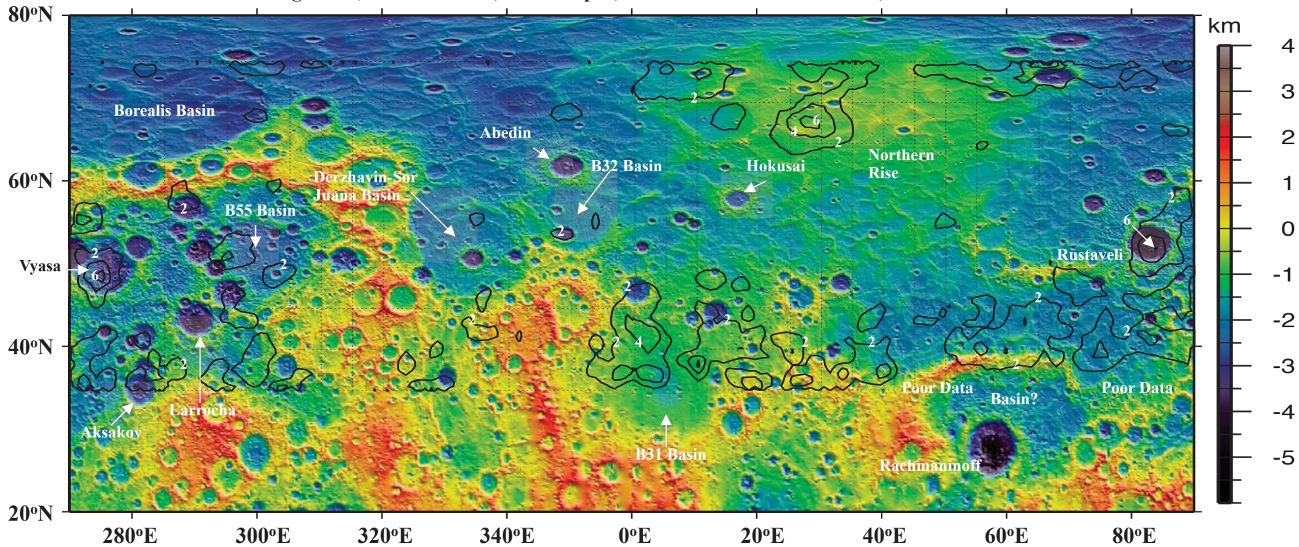
Field Magnitude, 40 km altitude; 20 km depth; mean rms deviation: 0.31 nT; Contour interval: 2 nT
