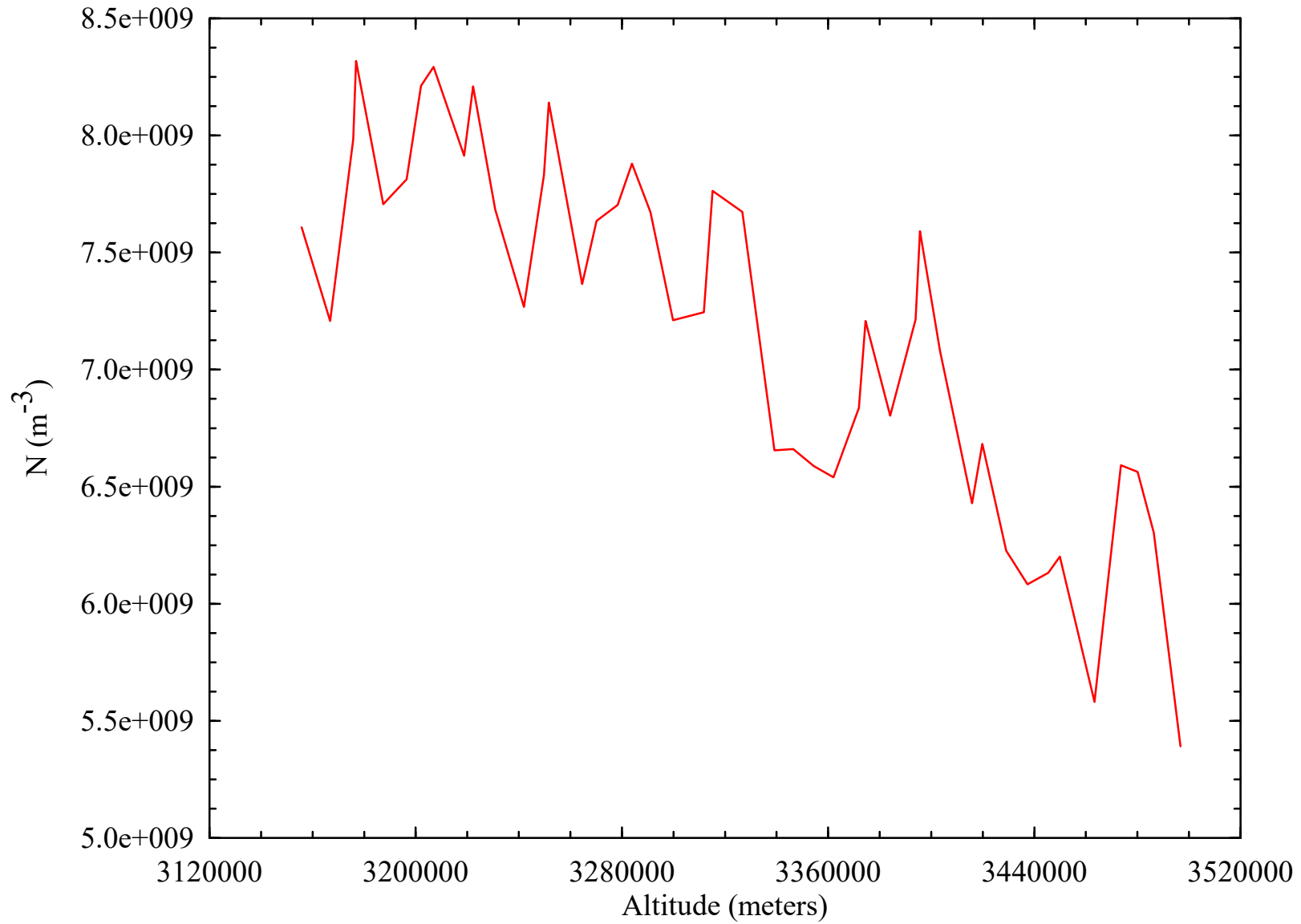
Electron Number Density vs. Altitude Derived from Jupiter Radio Occultation (J04_43XA)
