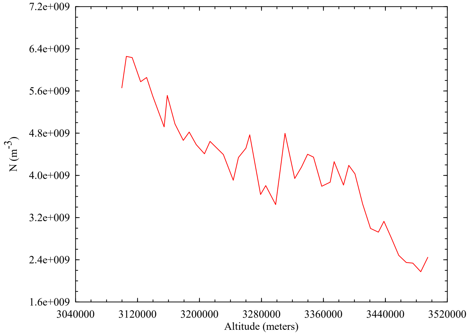
Electron Number Density vs. Altitude Derived from Jupiter Radio Occultation (J03_43NA)
