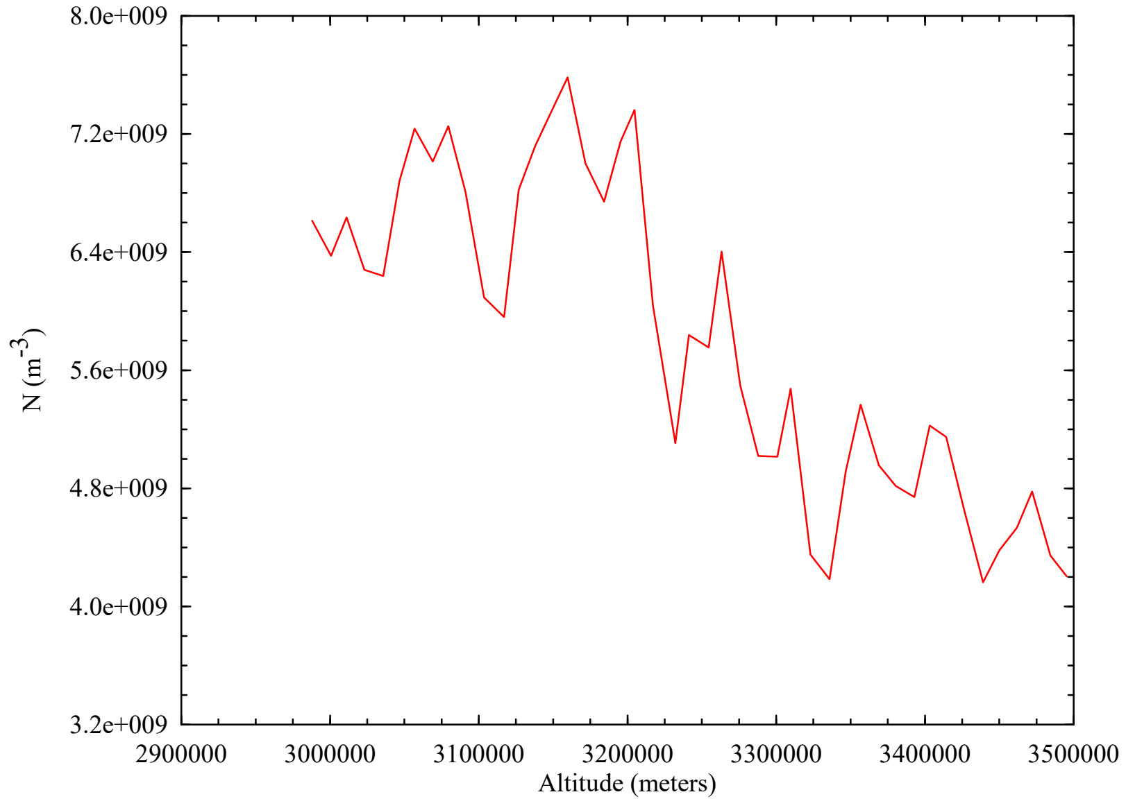
Electron Number Density vs. Altitude Derived from Jupiter Radio Occultation (J00_63XA)
