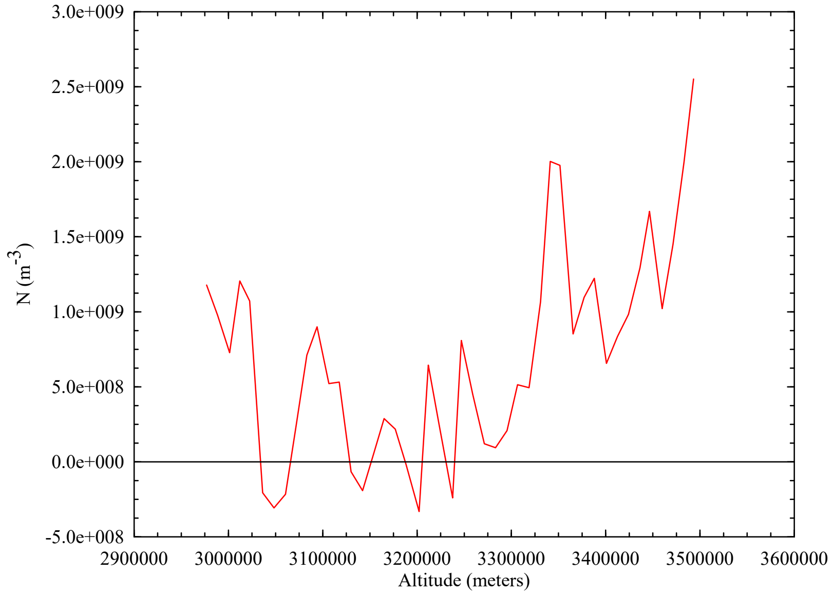
Electron Number Density vs. Altitude Derived from Jupiter Radio Occultation (J00_63NA)
