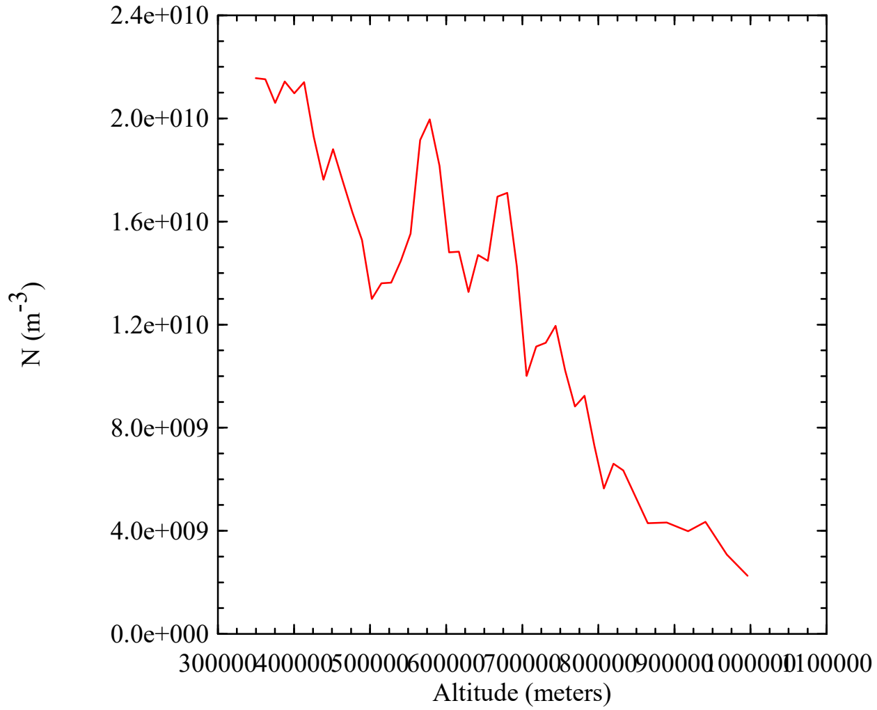
Electron Number Density vs. Altitude Derived from Io Radio Occultation (I09443NA)
