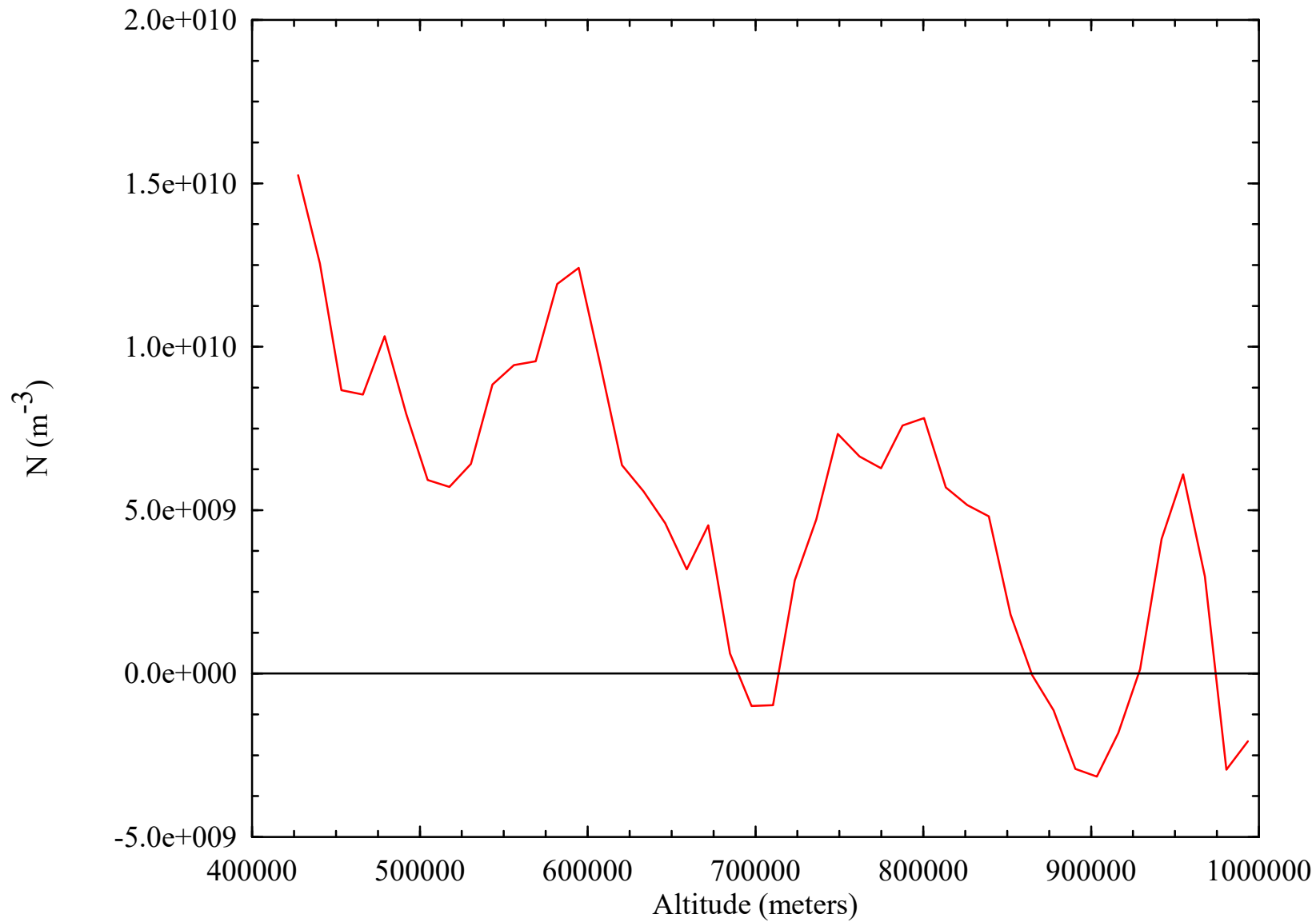
Electron Number Density vs. Altitude Derived from Io Radio Occultation (I09343NA)
