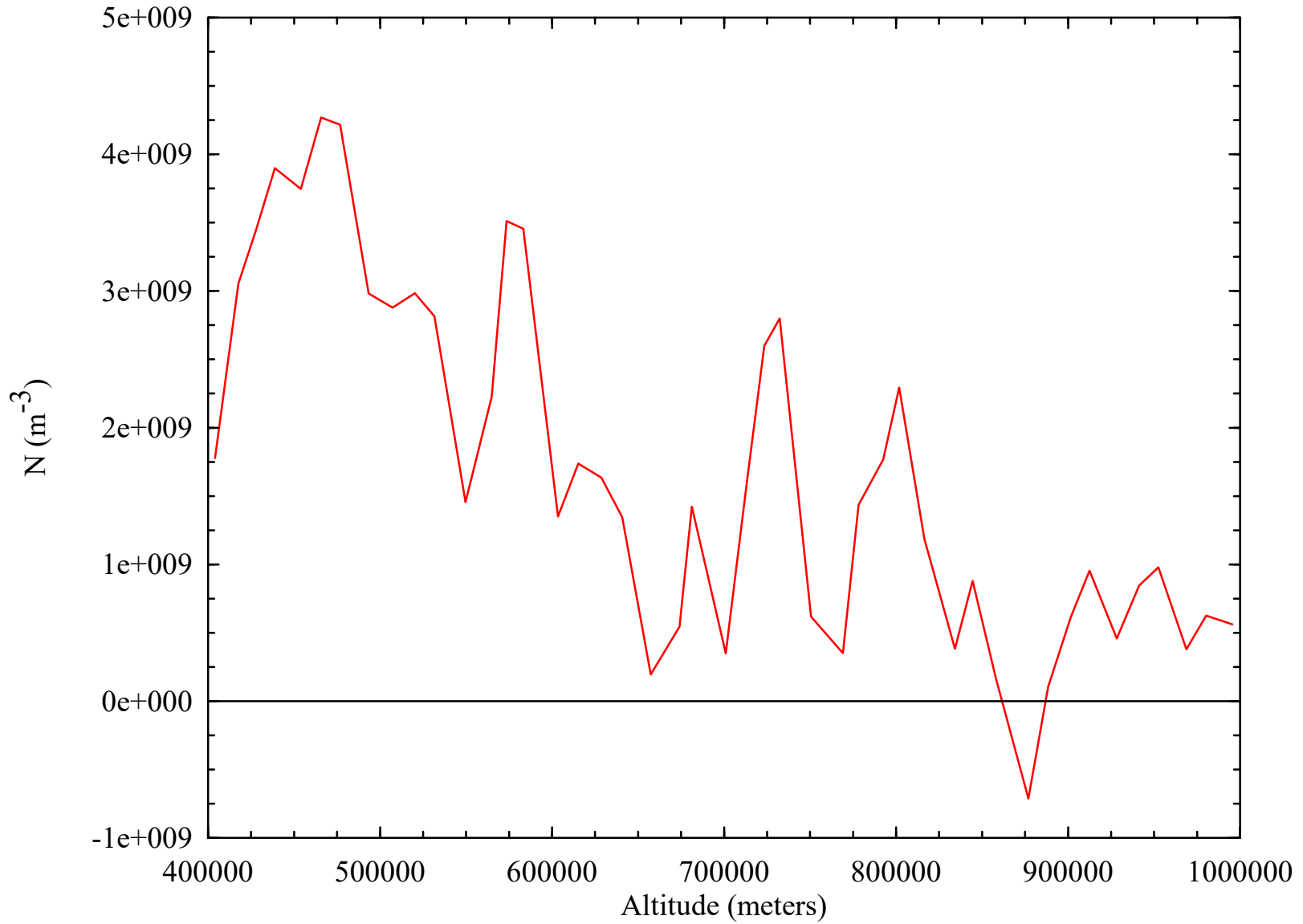
Electron Number Density vs. Altitude Derived from Io Radio Occultation (I09314XA)
