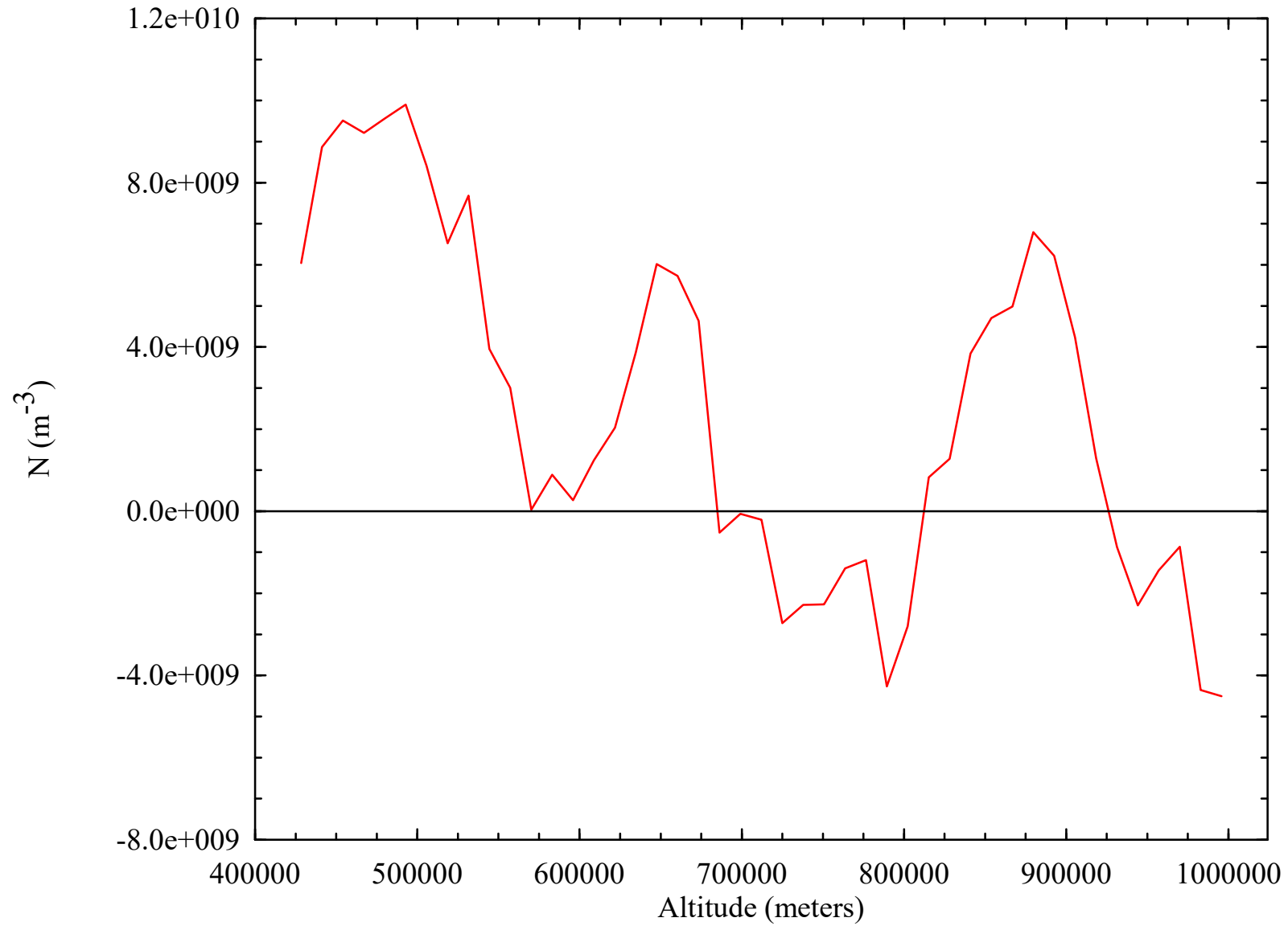
Electron Number Density vs. Altitude Derived from Io Radio Occultation (I09314NA)
