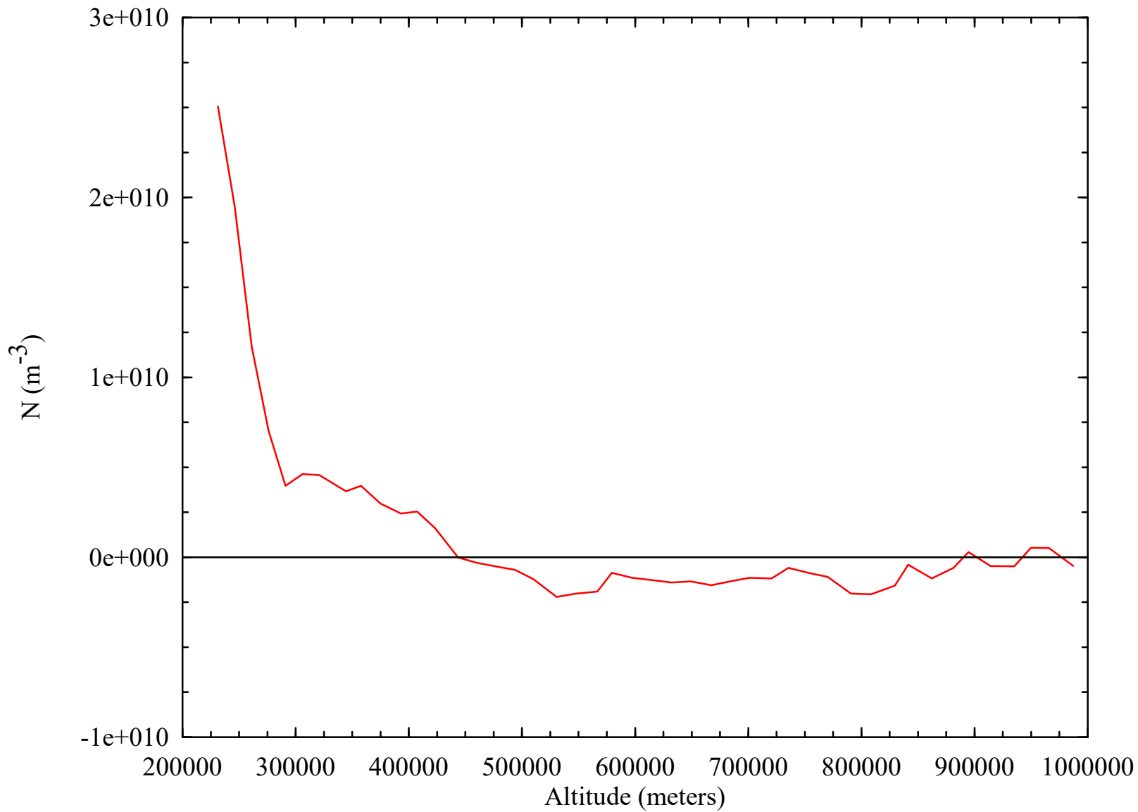
Electron Number Density vs. Altitude Derived from Io Radio Occultation (I09263XA)
