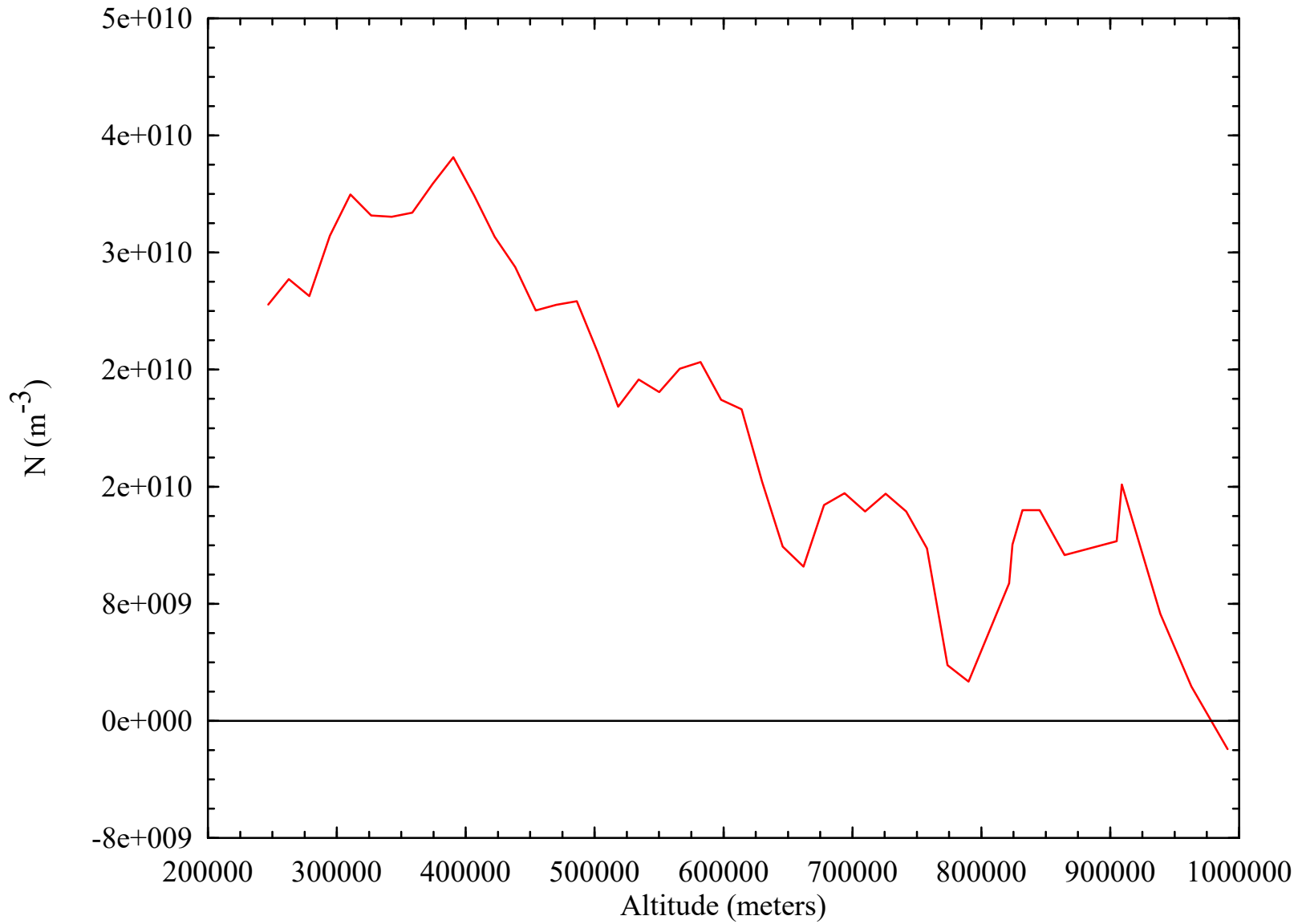
Electron Number Density vs. Altitude Derived from Io Radio Occultation (I09263NA)
