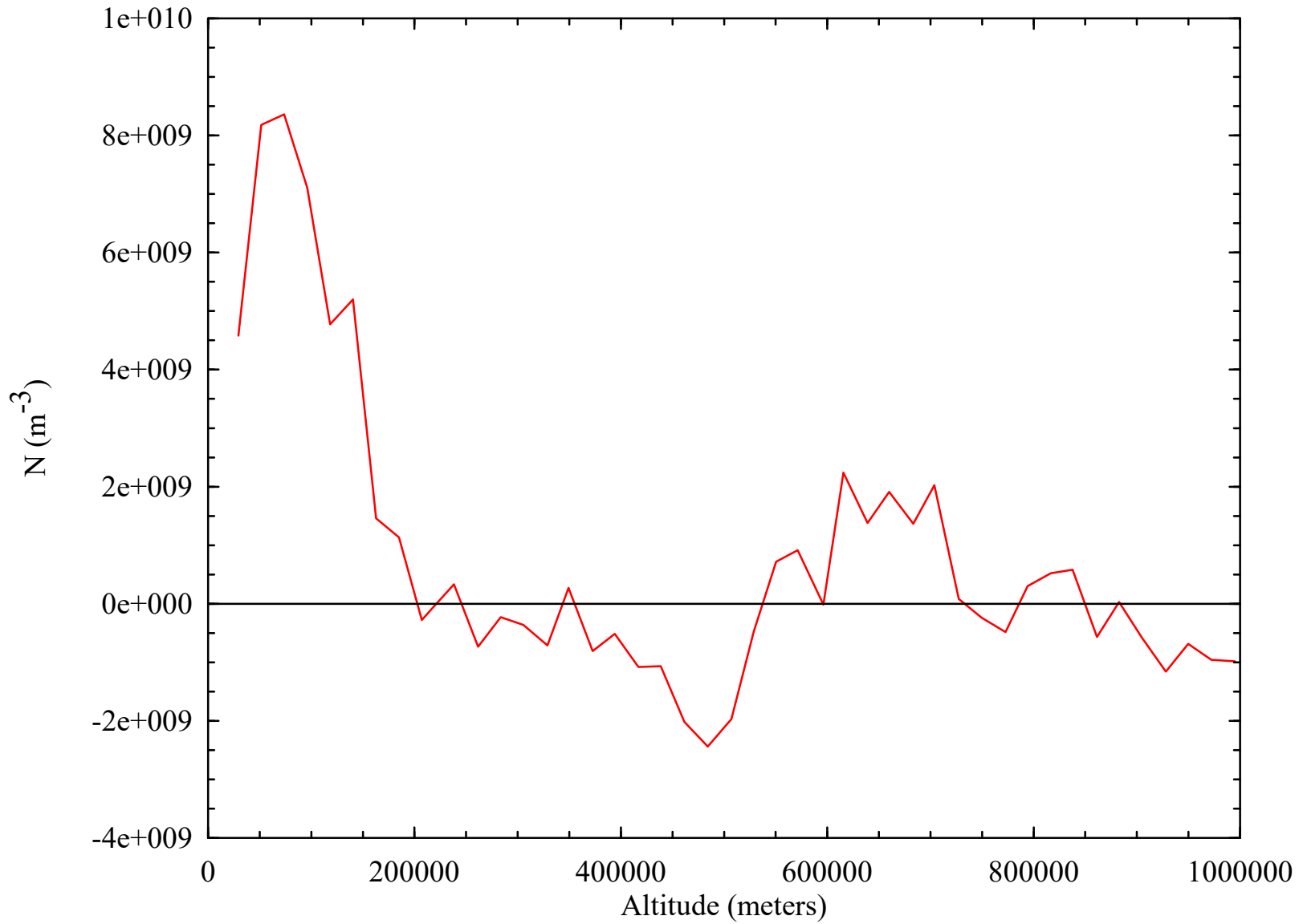
Electron Number Density vs. Altitude Derived from Io Radio Occultation (I06114XA)
