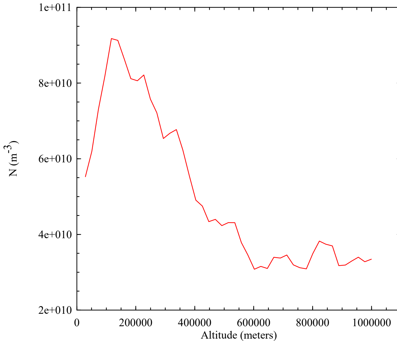
Electron Number Density vs. Altitude Derived from Io Radio Occultation (I06114NA)
