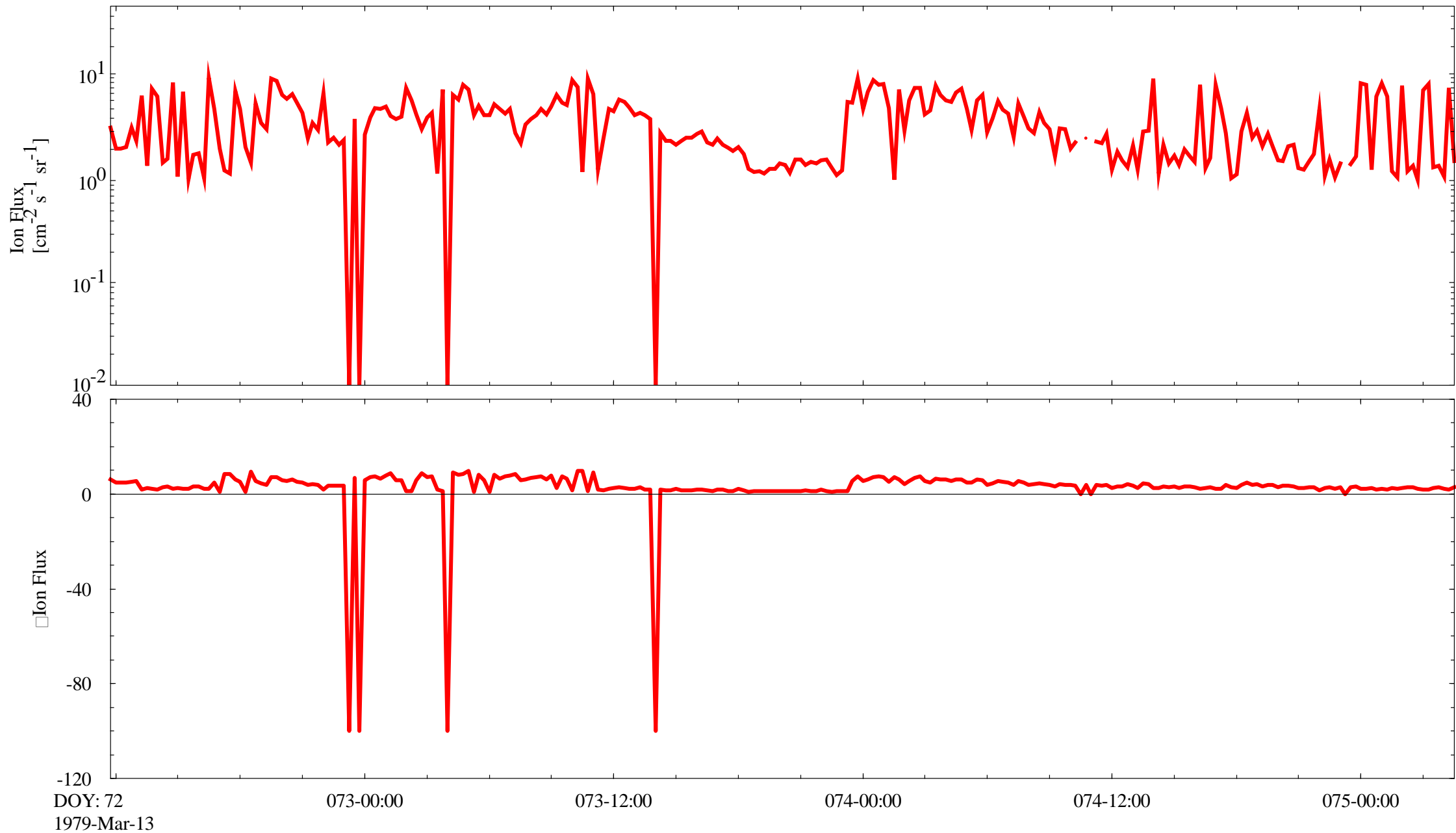
Voyager 1 CRS Proton Flux (1.8-8.1 MeV) from L[1] [2] [4] at Jupiter, Low Energy Telescope
