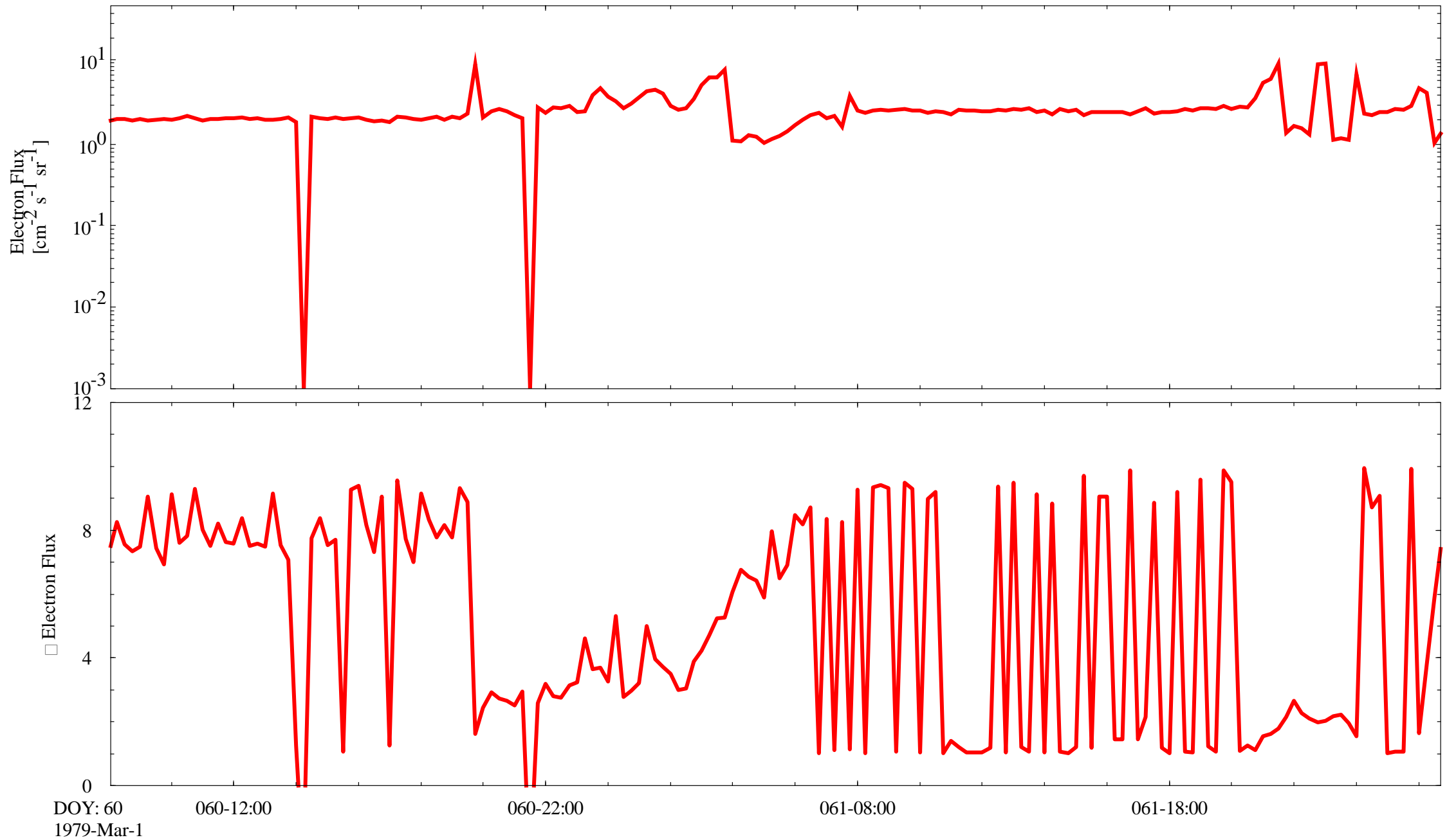
Voyager 1 CRS Electron Counting Rate (>0.5 MeV) at Jupiter from D[4], Electron Telescope
