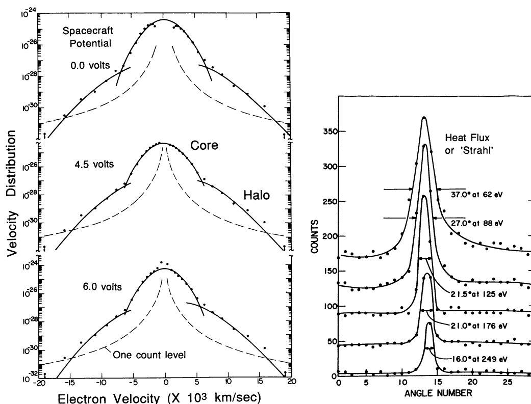
FIGURE 3. Bi-maxwellian fit to a typical solar wind electron velocity distribution (left panel), cut through along the magnetic field direction to show the existence of a low energy or 'core' component embedded in a higher energy but lower density 'halo' or 'strahl' component. A third "heat flux" component of electrons flowing out along the interplanetary field from the hot corona is illustrated on the right.
