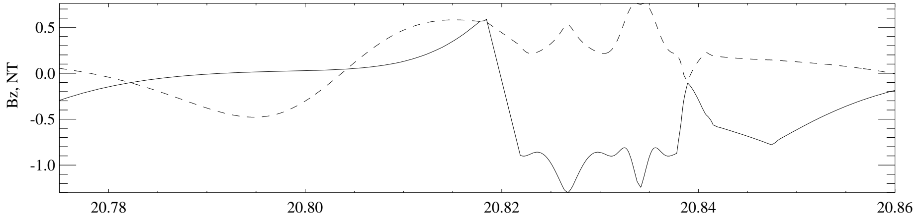
m00d020 Z - dashed ib_bsc_pl, solid ob_bsc_pl - 5 June 2000 model
