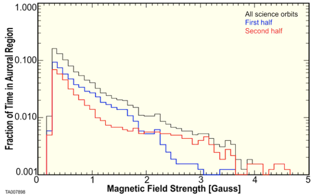
Fig. 8 Histograms of the estimated magnetic field strength that Juno is expected to encounter in the auroral regions
