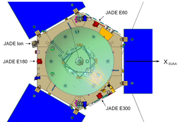
Fig. 5 Placement and FOVs of JADE-I and the three JADE-Es on the Juno spacecraft
