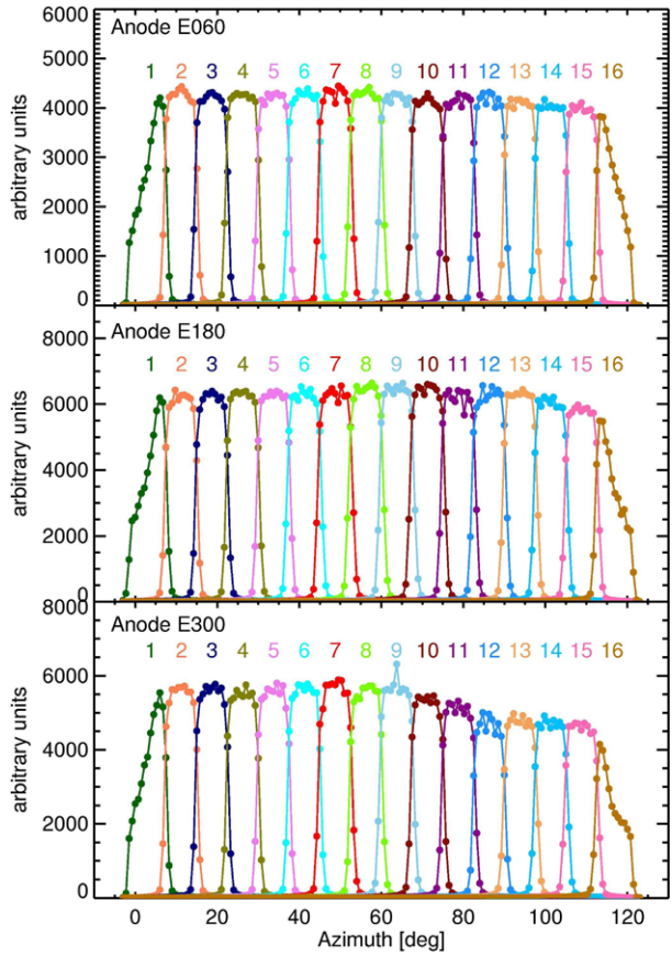
Fig. 53 Azimuthal angle response of all JADE-E sensors. (Note that there are no beam changes during calibration. Downward trend can be attributed to beam misalignment during sensor rotation; slight, off-transmission-peak variation ESA voltage; different efficiencies of MCP; or differences in FEE)
