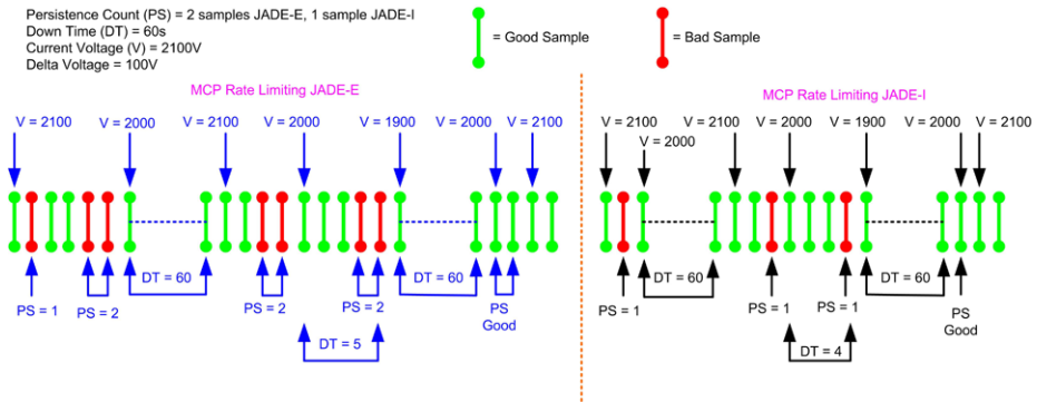
Fig. 77 MCP rate limiting algorithm
