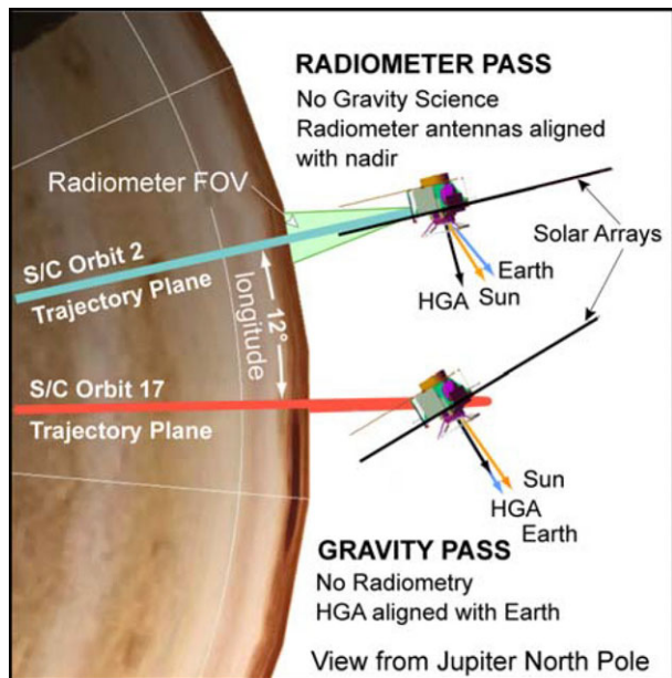
Fig. 70 Juno attitude for radiometer (MWR) and gravity (GRAV) orbits
