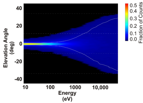
Fig. 61 Modeled distributions of the elevation angles as a function of energy. In this model, no angular scattering or energy straggling effects were included. Also it was assumed that all ions pass through the foils with a neutral charge state. Since including realistic scattering and electronic effect will further scatter the ions paths, this result should be interpreted as a limiting case of the angular response
