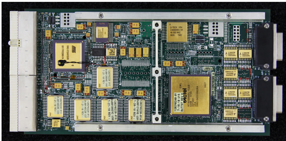
Fig. 30 Instrument Processor Board (IPB)
