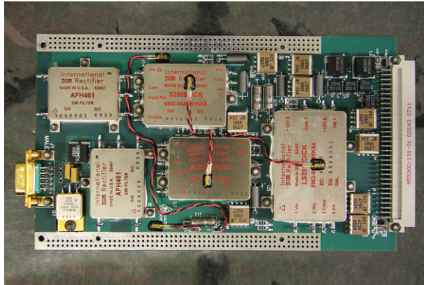
Fig. 32 Low Voltage Power Supply Board
