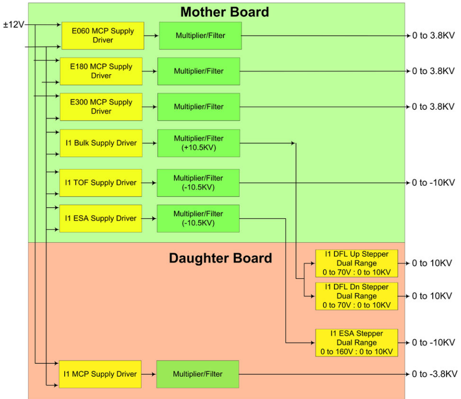
Fig. 38 HVPS Board 2 block diagram
