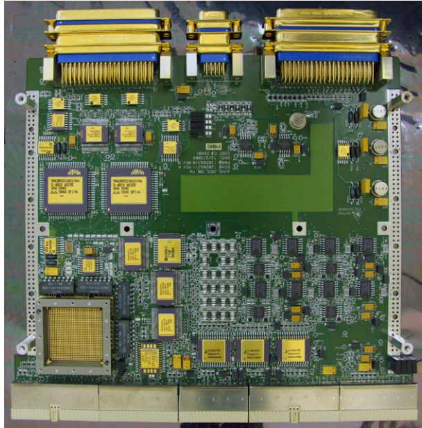
Fig. 36 JADE Sensor Interface Board photograph
