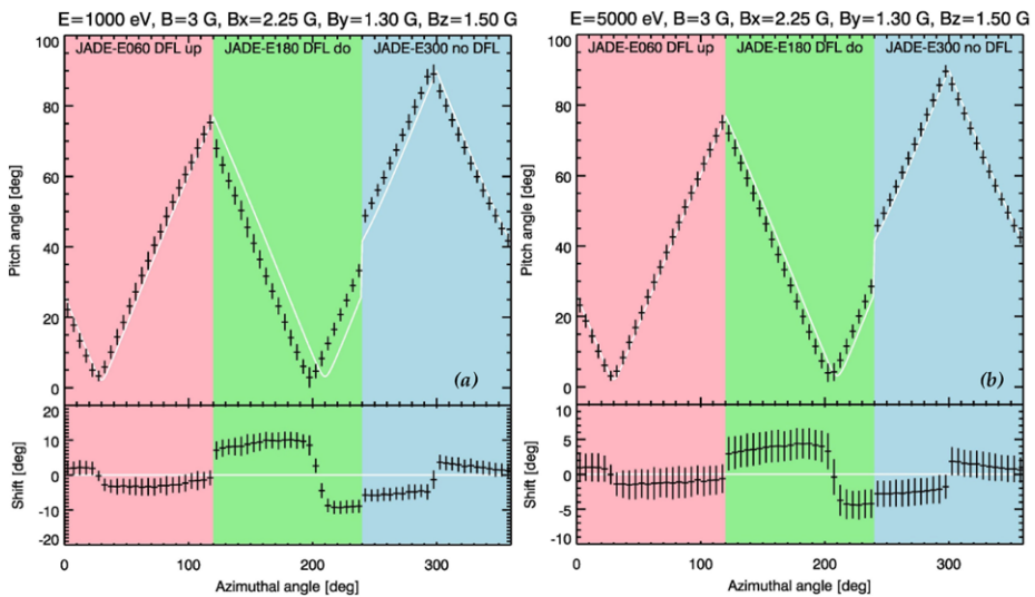
Fig. 9 Simulations of pitch-angle deflection of (a) 1 keV and (b) 5 keV electrons after passing through the ESA of the JADE-E sensor in an external magnetic field strength of B_X = 2.25 G, B_Y = 1.3 G, B_Z = 1.5 , and B = 3 G. The white curve is undeflected pitch angle. The bottom panels show the angular shift
