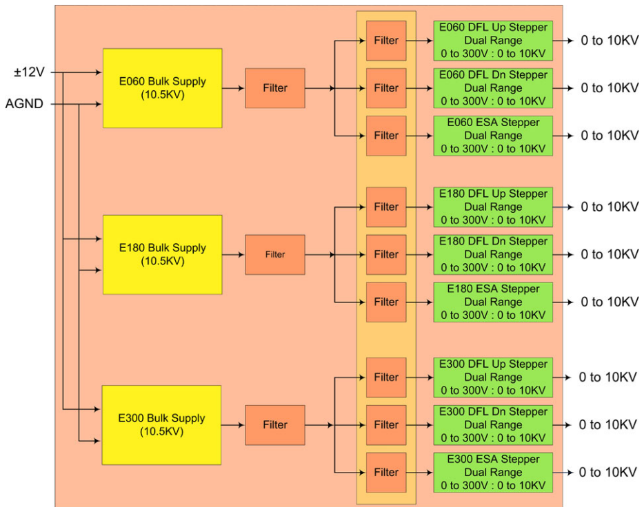
Fig. 37 HVPS Board 1 block diagram
