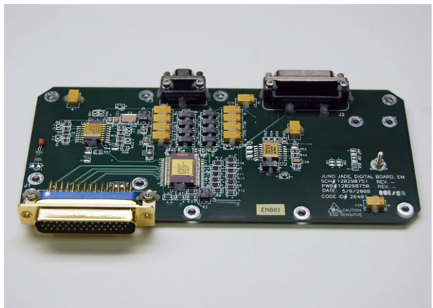
Fig. 19 JADE-E Digital Board
