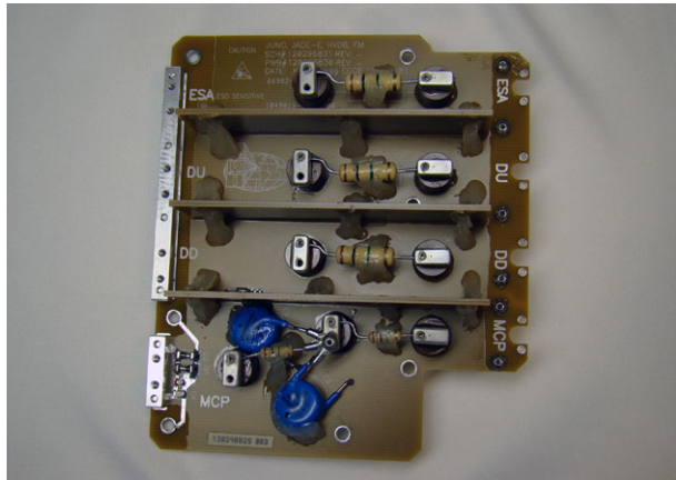
Fig. 21 JADE-E High Voltage Distribution Board (HVDB)
