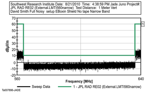
Fig. 2 Example of MWR notch EMI result for JADE
