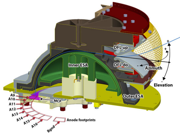
Fig. 6 Schematic diagram of the JADE-E sensor
