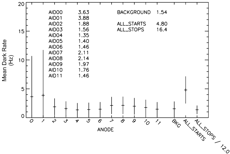
Fig. 68 Dark rate observed in the JADE-I sensor during flight calibration. The mean dark rate for each anode is indicated by the horizontal line, and the vertical line is \pm 1\sigma
