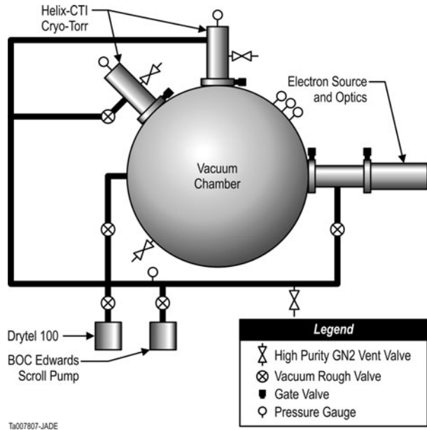
Fig. 84 Schematic of the electron calibration facility vacuum components. Only oil-free vacuum pumps are used in this system to minimize the possibility of contamination to the instruments under test. Cleanliness of the vacuum is monitored with a 200 amu Residual Gas Analyzer (RGA)
