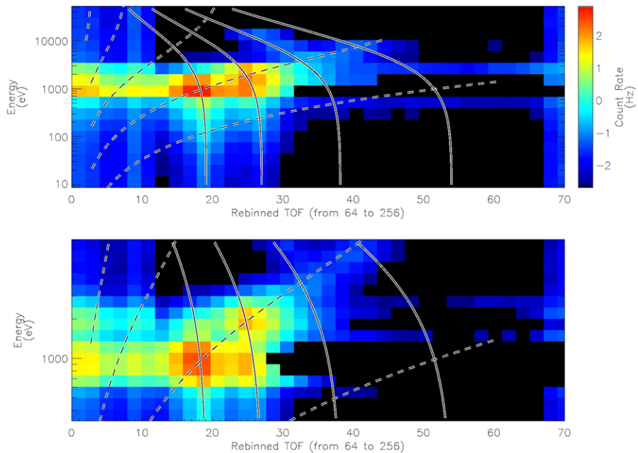
Fig. 82 Energy–TOF spectrograms for two different sweep tables. Overplotted on the data are curves of constant M/q (solid lines) and constant incident velocity (dashed lines). The top panel shows data for sweep table 1, which covers from 10 eV–40 keV (the same energy steps as used during HRS mode and shown in Fig. 81). The bottom panel shows data for sweep table 2, which covers the typical solar wind energies of 0.3–8 keV
