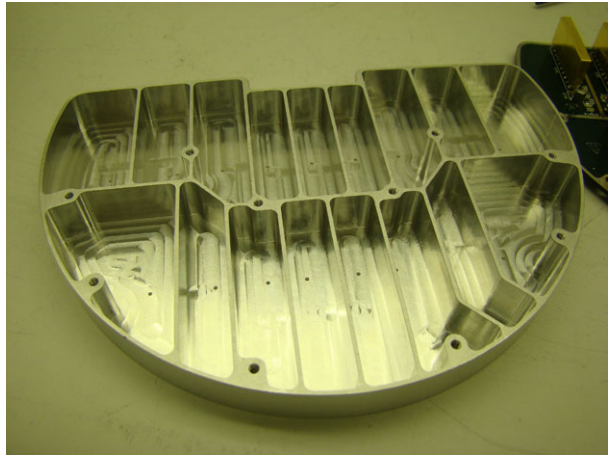
Fig. 18 JADE-E Board stiffener/electro-static isolation housing
