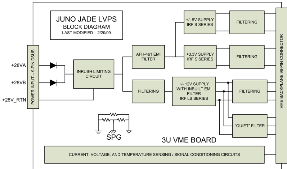
Fig. 33 LVPS block diagram
