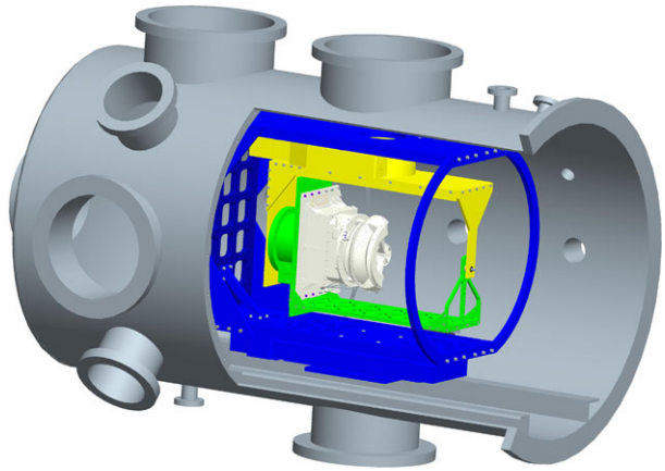
Fig. 85 Cut away of main vacuum vessel showing the three stages of the positioning system: horizontal translation stage (blue), outer rotation stage (yellow), and inner rotation stage (green). For reference, a JADE-E sensor (white) is shown mounted onto the positioning system
