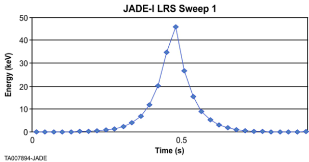
Fig. 75 One JADE-I LRS/Cal ESA sweep
