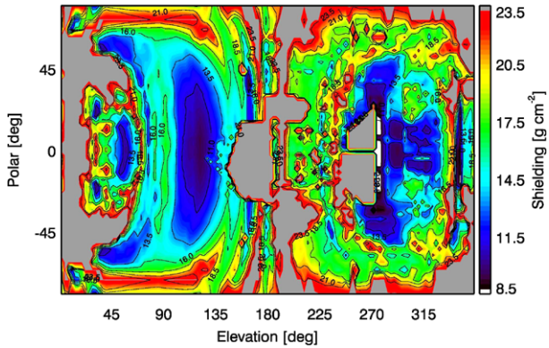
Fig. 46 Rectangular projection of the JADE-E radiation shielding thickness viewed from Anode 8
