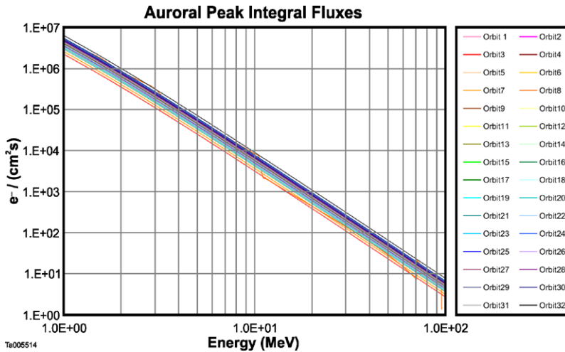
Fig. 41 Peak integral fluxes from the auroral region for all orbits (note that orbit numbering here starts with the first complete 11-day orbit). Since the auroral region is in L -shells > 6 , the JPL-DG model was used to calculate integral fluxes. The SwRI-DSC model was applied only to orbit segments where L < 6
