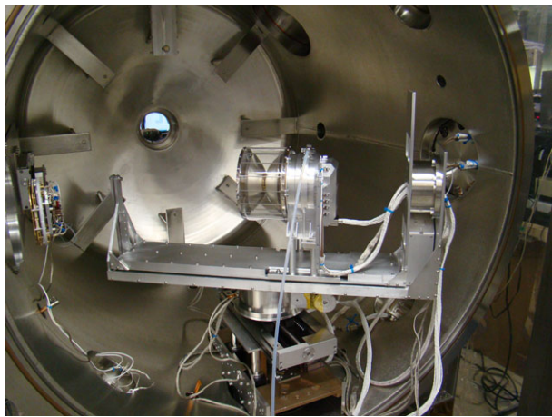
Fig. 58 The JADE-I sensor mounted for calibration on a 4-axis positioning system, which allows illumination of the full FOV
