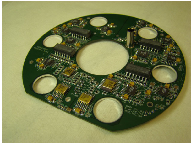
Fig. 25 JADE-I TOF Board
