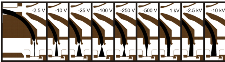
Fig. 11 Simulated exit trajectories for ions passing through the JADE-I ESA. The ESA voltage is varied a range of values, from -2.5 V to -10 kV. The carbon foil is at -10 kV and deflectors are at 0 V for all these runs
