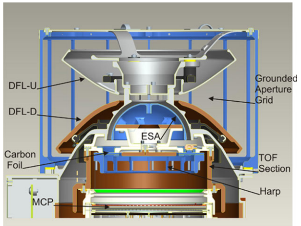
Fig. 10 Cross section of the JADE-I electro-optics
