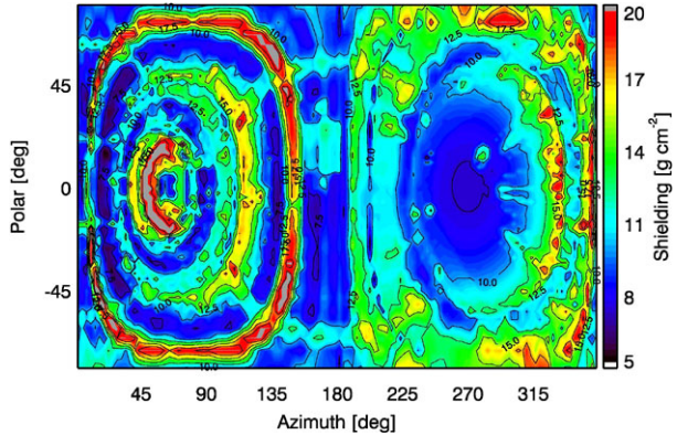
Fig. 45 Rectangular projection of the JADE-I radiation shielding thicknesses as viewed from Anode 6
