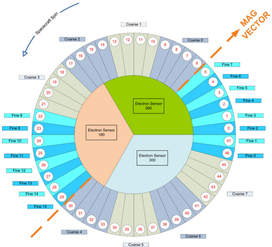
Fig. 71 JADE-E data collapse based on broadcast magnetic field data
