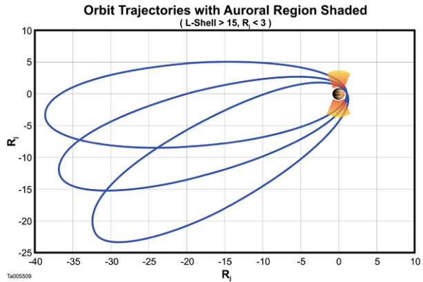
Fig. 39 Juno's trajectory for orbits at the start ( horizontal ), middle, and end ( highly inclined ) of the nominal science mission. The yellow-shaded portions roughly indicate periods when Juno is in the auroral region (see text for details)
