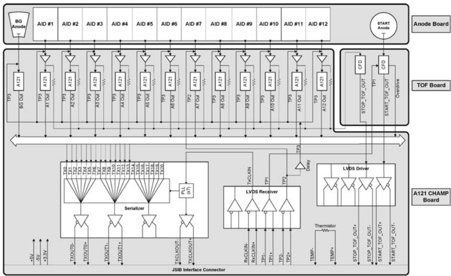
Fig. 23 Overview of the JADE-I Charge Amplifier and TOF Boards
