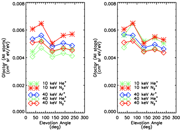
Fig. 65 Geometric factor measured during calibration includes detector efficiency. The dip seen at 135^\circ is where the ion beam is incident at an angle between two anodes and mechanical structures in the instrument partially obscure the beam
