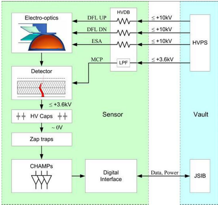
Fig. 14 JADE-E Sensor Electronics block diagram
