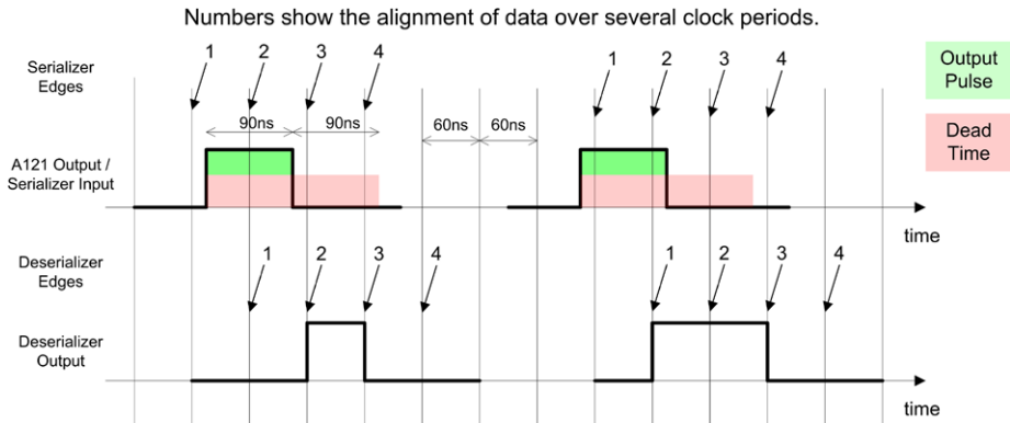
Fig. 20 JADE-E Digital Board timing diagram
