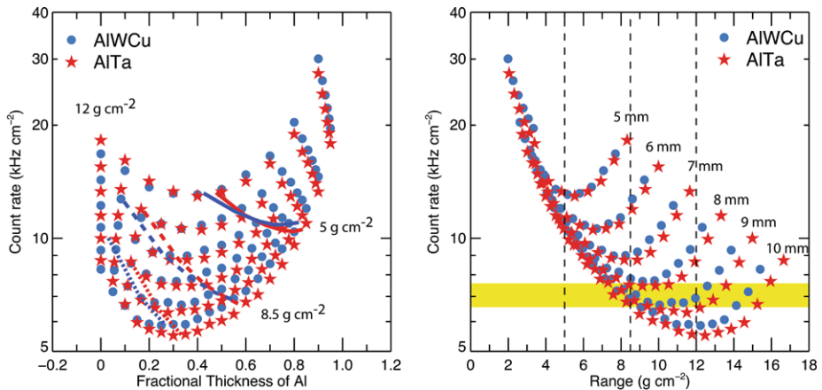
Fig. 42 Estimated MCP count rate plotted vs. (a) the fractional thickness of Al, and (b) the stopping power of the graded-Z shield
