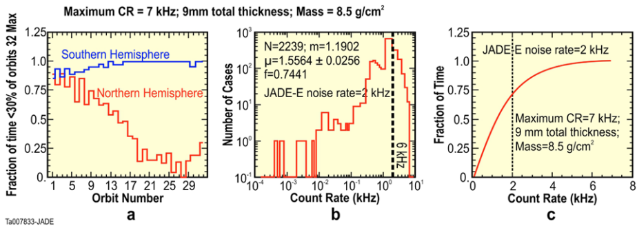
Fig. 44 Similar to Fig. 43, but for JADE-E and using a 9-mm thick shield with a stopping power of 8.5 \text{ g/cm}^2
