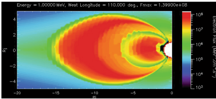
Fig. 40 Differential fluxes from the SwRI-DSC physical model for L < 6 and the JPL-DG model for L > 6 . The differences between the physical model and JPL code for L < 6 are significant only in relation to the differential fluxes; the simulation results from the two models are similar in terms of the integral flux
