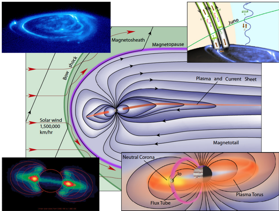
Fig. 1 The magnetosphere of Jupiter
