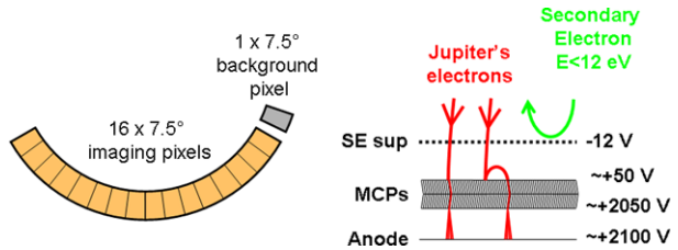
Fig. 7 Schematic of the JADE-E detector. A cross section is shown on the right-hand side and a view of the imaging anodes and the background anode on the left-hand side
