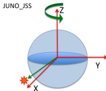
Figure 12: The Jupiter De-Spun-Sun (JUNO_JSS) co-ordinate system.
