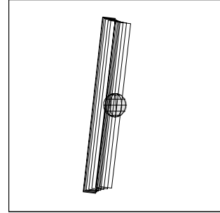
24IUSURFAC02 IEE+CDS 1080:00:0 99-284/22:44:57
