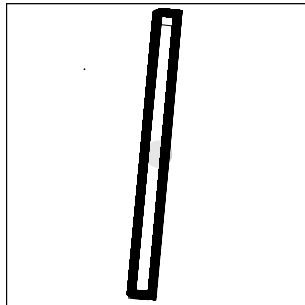
24IUECLIPS01 99-285/03:08:51
