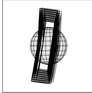
24IUATMOS_02 IEE+CDS 806:00:0 99-284/18:07:54
