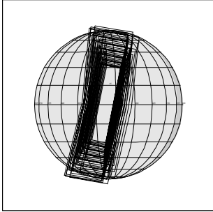
24IUATMOS_01 IEE+CDS 438:00:0 99-284/11:55:49
