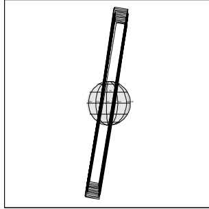
24IUSURFAC01 IEE+CDS 712:00:0 99-284/16:32:52
