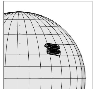
24IPREGMAP01 99-284/05:57:49
