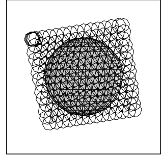
24IPGLOBAL02 99-283/16:00:41
