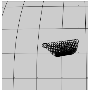
24IPLOKI_02 99-284/03:41:23
