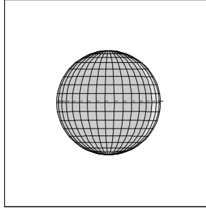
24IPGLOBAL01 99-283/15:30:21
