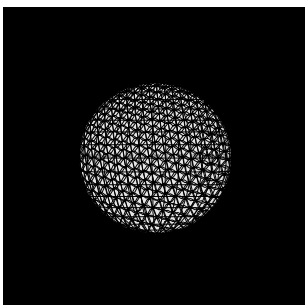
24IPGLOBAL04 99-284/09:19:02
