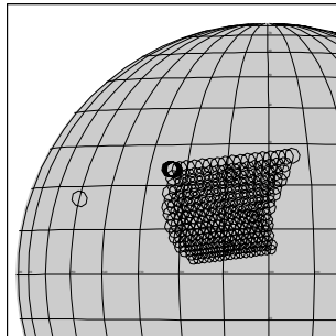
24IPLOKI_01 99-284/02:55:53
