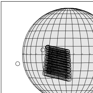
24IPREGMAP02 99-284/06:52:29
