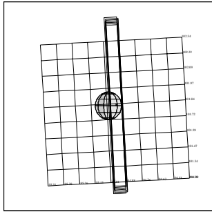
15EUATMOS_01 JEE-CDS 1696:00:0 98-150/21:59:37
