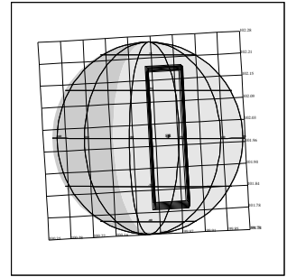
15EUSURFAC01 JEE-CDS 1058:00:0 98-151/08:44:42
