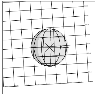
15IUHRSPEC01 JEE-CDS 459:00:0 98-151/13:14:40
