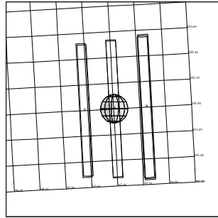
15EUATMOS_02 JEE-CDS 1512:00:0 98-151/01:05:39
