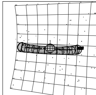
15TU15MANS01 98-153/18:31:44
