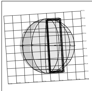
15IUSURFAC01 JEE-CDS 851:00:0 98-151/12:14:00
