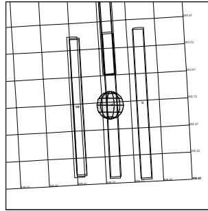
15IUATMOS_01 JEE-CDS 1182:00:0 98-151/06:39:19
