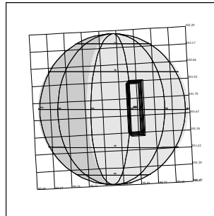
15EUSURFAC02 98-151/14:14:19
