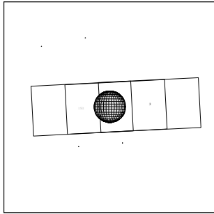
15ISHIPHAS01 IEE-CDS 1250:00:0 98-150/23:54:53
