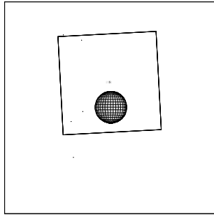
15ISECLIPS01 IEE-CDS 1231:00:0 98-151/00:14:05
