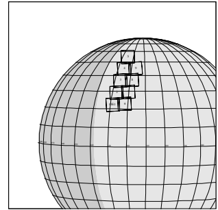
15ESREGMAP01 EEE-CDS 65:00:0 98-151/20:07:12
