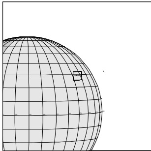
15ESPHOTOM01 EEE-CDS 59:00:0 98-151/20:13:16
