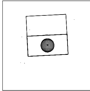
15ISECLIPS02 IEE-CDS 1198:00:0 98-151/00:47:27
