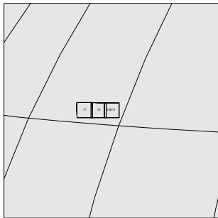
15ESRELIEF02 98-151/21:12:55
