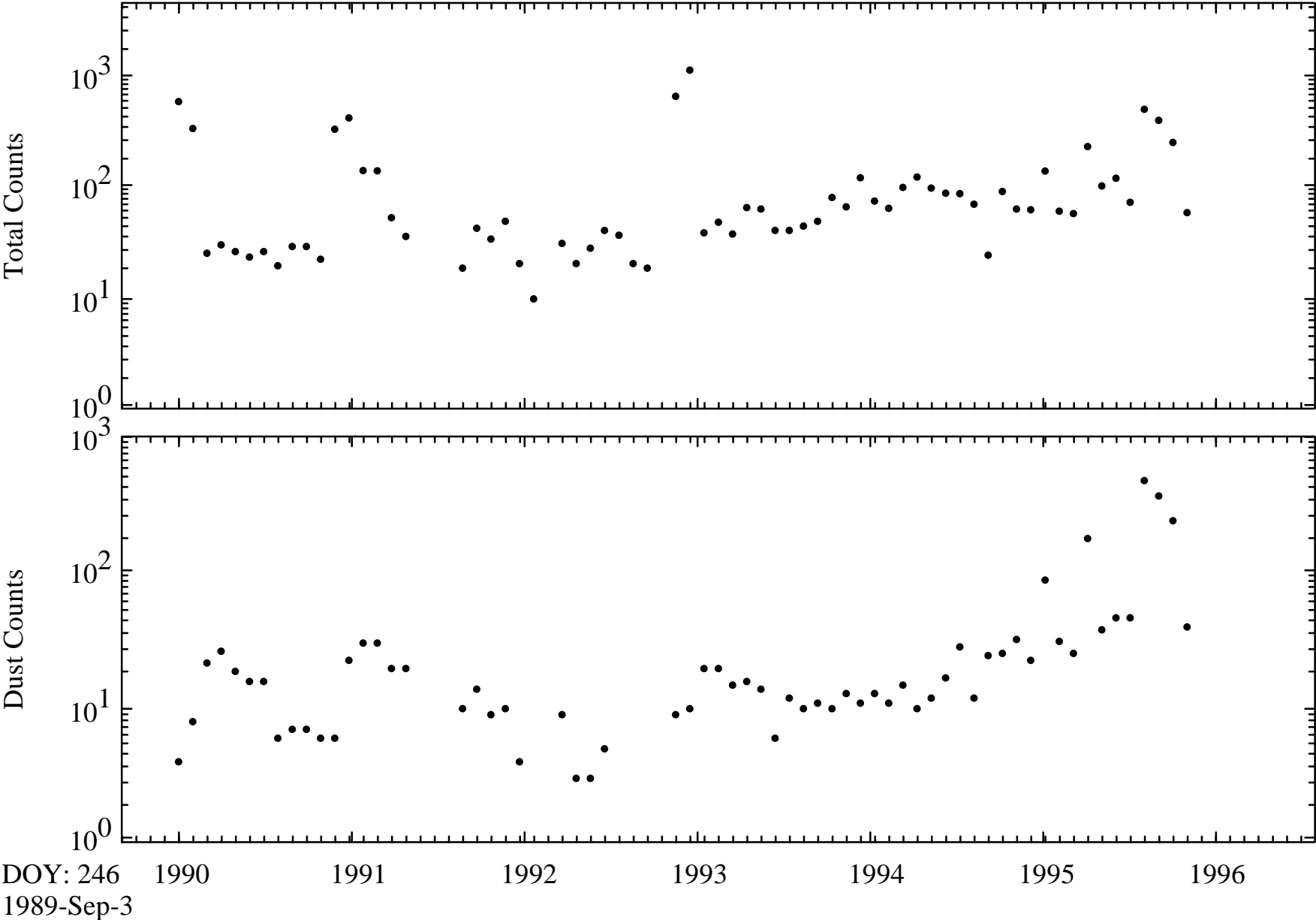
Pre-Jupiter Total and Dust Counts vs Time
