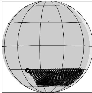
25IPREGMAP01 IEE-CDS 131:00:0 99-330/01:53:04
