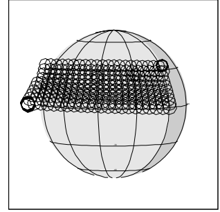
25EPH2O40_02 EEE+CDS 138:00:0 99-329/18:48:20
