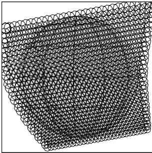
25IPGLOBAL01 IEE-CDS 312:00:0 99-329/22:50:03
