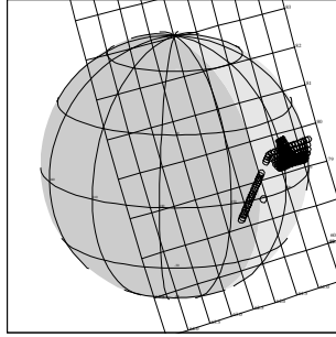
25EPH2O12001 EEE-CDS 45:00:0 99-329/15:43:22
