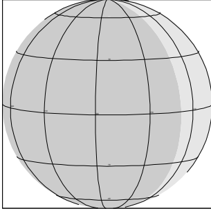
25EPDRKMAP01 EEE-CDS 137:00:0 99-329/14:10:21
