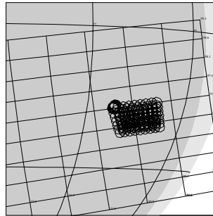
25IPPELE_01 IEE-CDS 56:00:0 99-330/03:08:54
