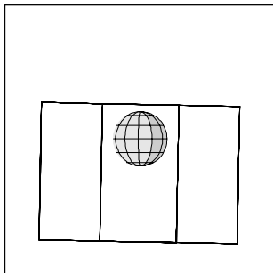
14ISECLIPS01 IEE+CDS 1280:00:0 98-089/02:22:27
