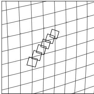
14ESDRKSPT01 EEE-CDS 3:00:0 98-088/13:17:50
