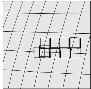
14ESTRPBND01 EEE+CDS 6:40:0 98-088/13:27:23
