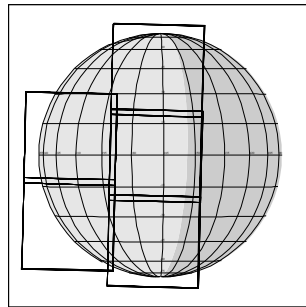
14ESGLOCOL01 EEE+CDS 356:00:0 98-088/19:20:49
