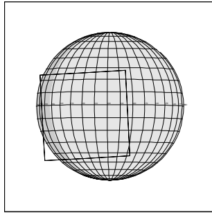
14ISCONTEX01 IEE-CDS 110:00:0 98-088/02:57:01
