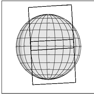
14ISPOLAR_01 IEE-CDS 258:00:0 98-088/00:27:22
