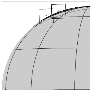
11JSAURORA01 JEE-CDS 1786:00:0 97-309/18:35:45
