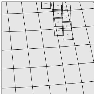
11ESMORPHY01 EEE+CDS 6:00:0 97-310/20:37:56
