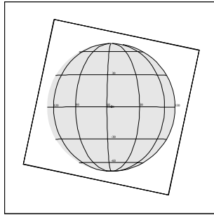
11CSPHOTOM01 CEE+CDS 208:00:0 97-309/10:46:36
