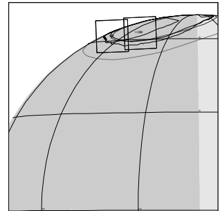
11JSAURORA03 JEE-CDS 1693:00:0 97-309/20:09:47
