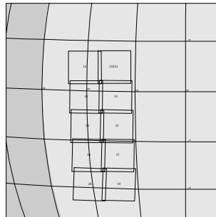
11ESREGMAP01 EEE-CDS 70:00:0 97-310/19:21:05
