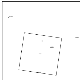
11SSAMALTH01 JEE+CDS 15:00:0 97-311/00:56:46
