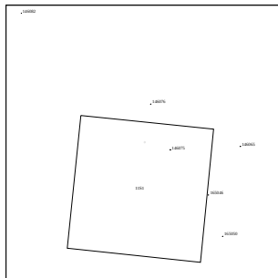
11SSTHEBE_01 JEE-CDS 68:00:0 97-310/23:32:51
