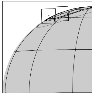
11JSAURORA02 JEE-CDS 1740:00:0 97-309/19:22:16
