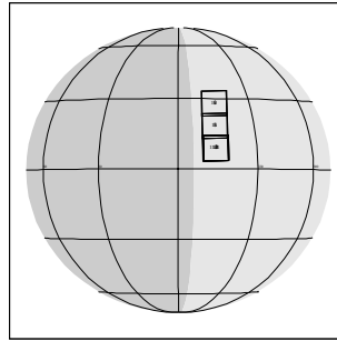
11JSFEATRK01 JEE-CDS 1923:00:0 97-309/16:17:14
