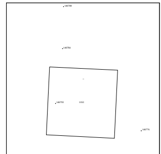
11SSADRAST01 JEE+CDS 117:00:0 97-311/02:39:54
