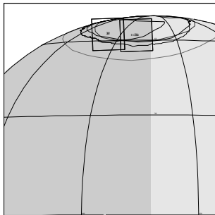
11JSAURORA04 JEE-CDS 1647:00:0 97-309/20:56:18
