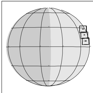
11JSFEATRK03 JEE-CDS 1839:00:0 97-309/17:42:10
