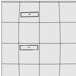
11ESCOLORS01 EEE-CDS 88:00:0 97-310/19:02:53
