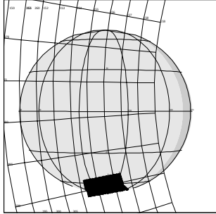
C9JNSPOLEM05 97-178/16:44:42
