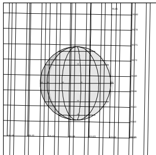
C9ENRTECLI01 97-177/16:06:28
