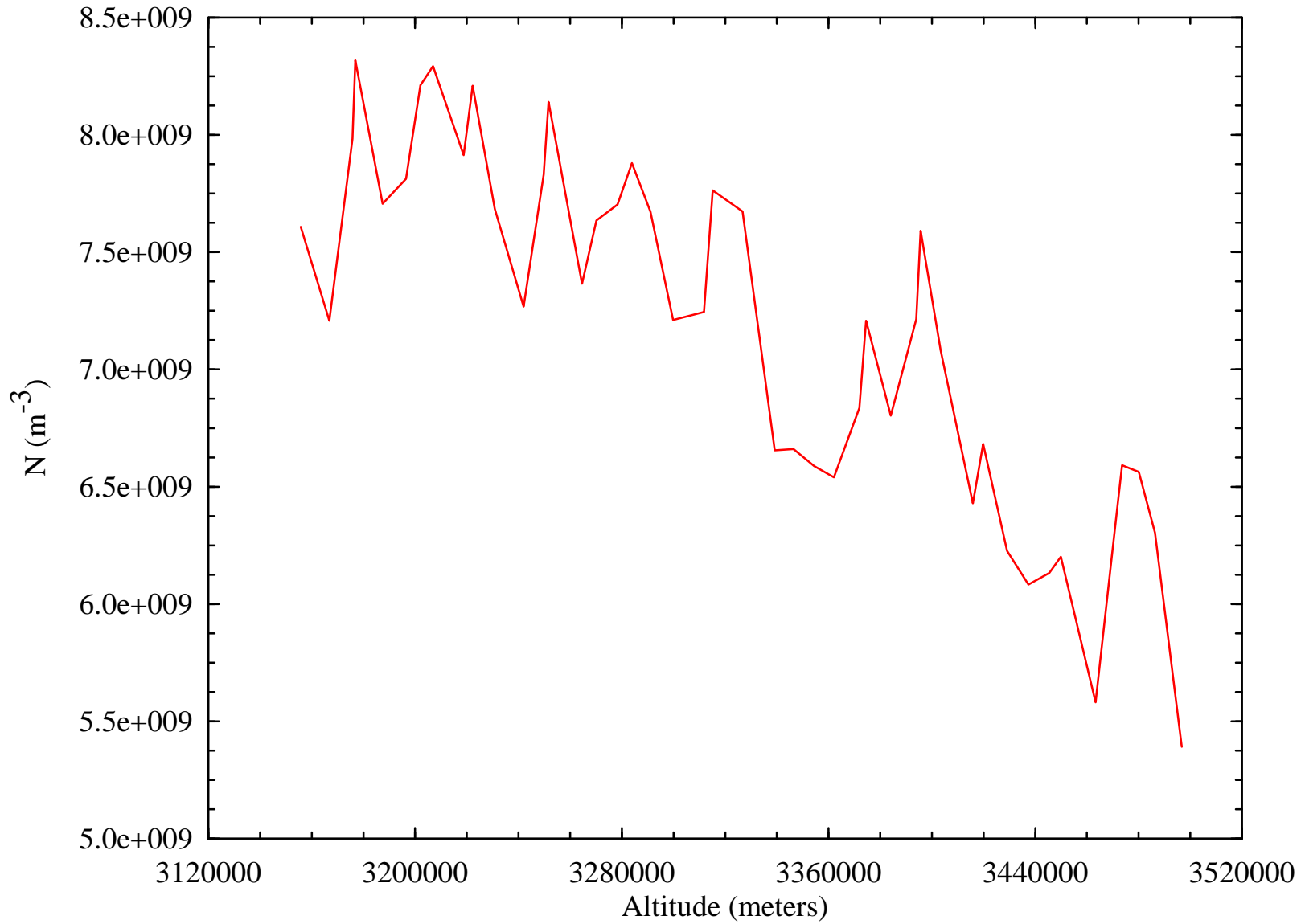
Electron Number Density vs. Altitude Derived from Io Radio Occultation (J04_43XA)
