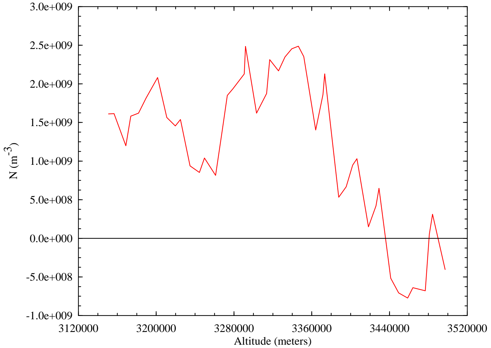
Electron Number Density vs. Altitude Derived from Io Radio Occultation (J04_14NA)
