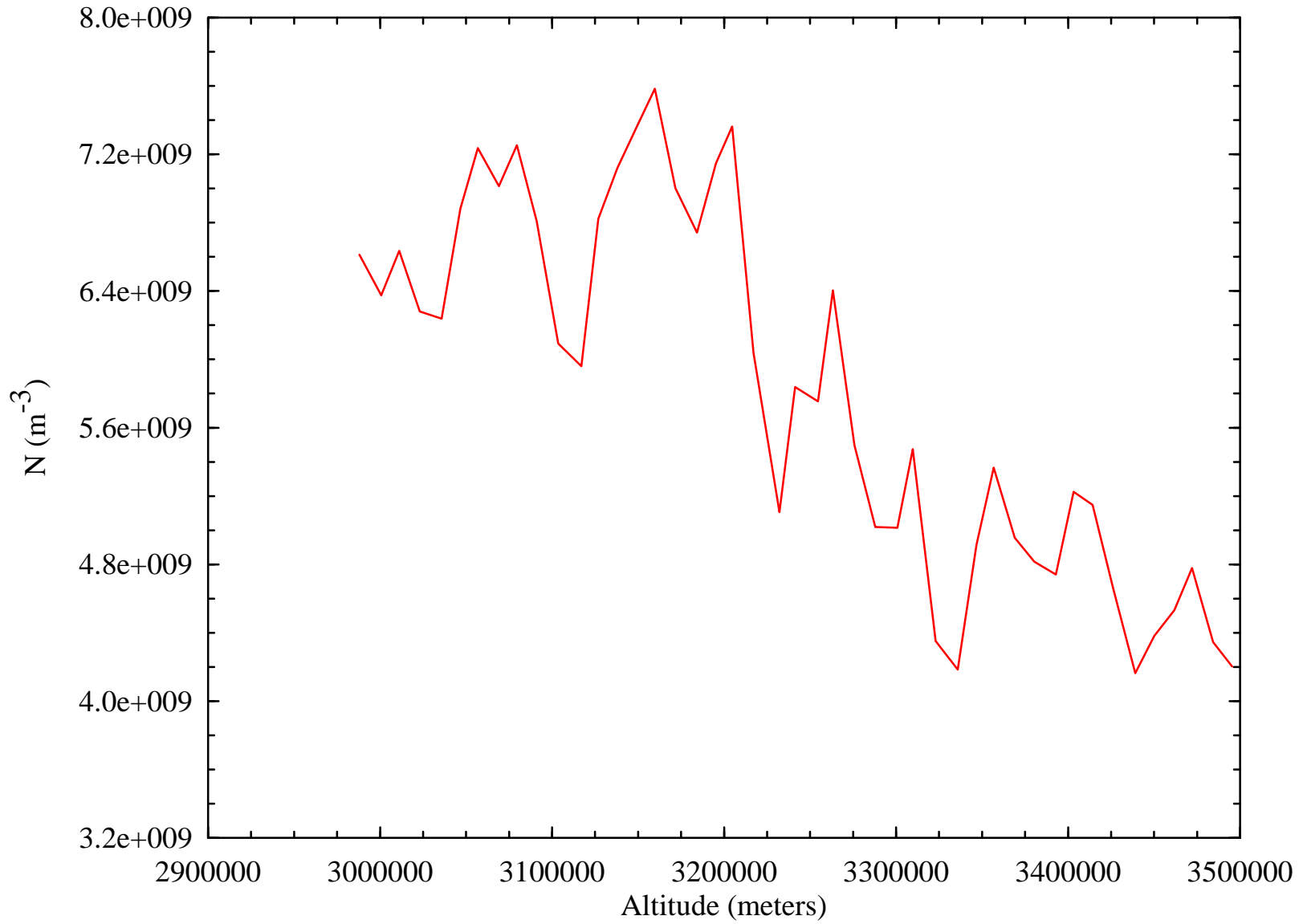
Electron Number Density vs. Altitude Derived from Io Radio Occultation (J00_63XA)
