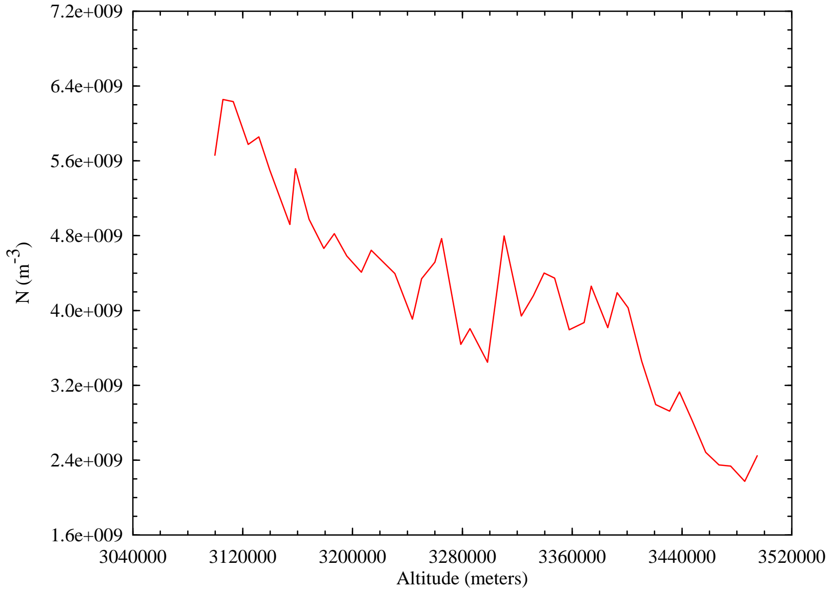
Electron Number Density vs. Altitude Derived from Io Radio Occultation (J03_43NA)
