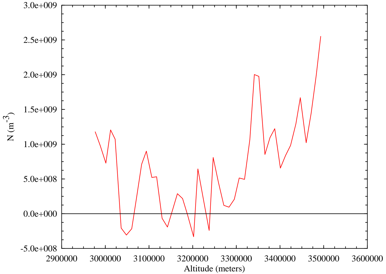
Electron Number Density vs. Altitude Derived from Io Radio Occultation (J00_63NA)
