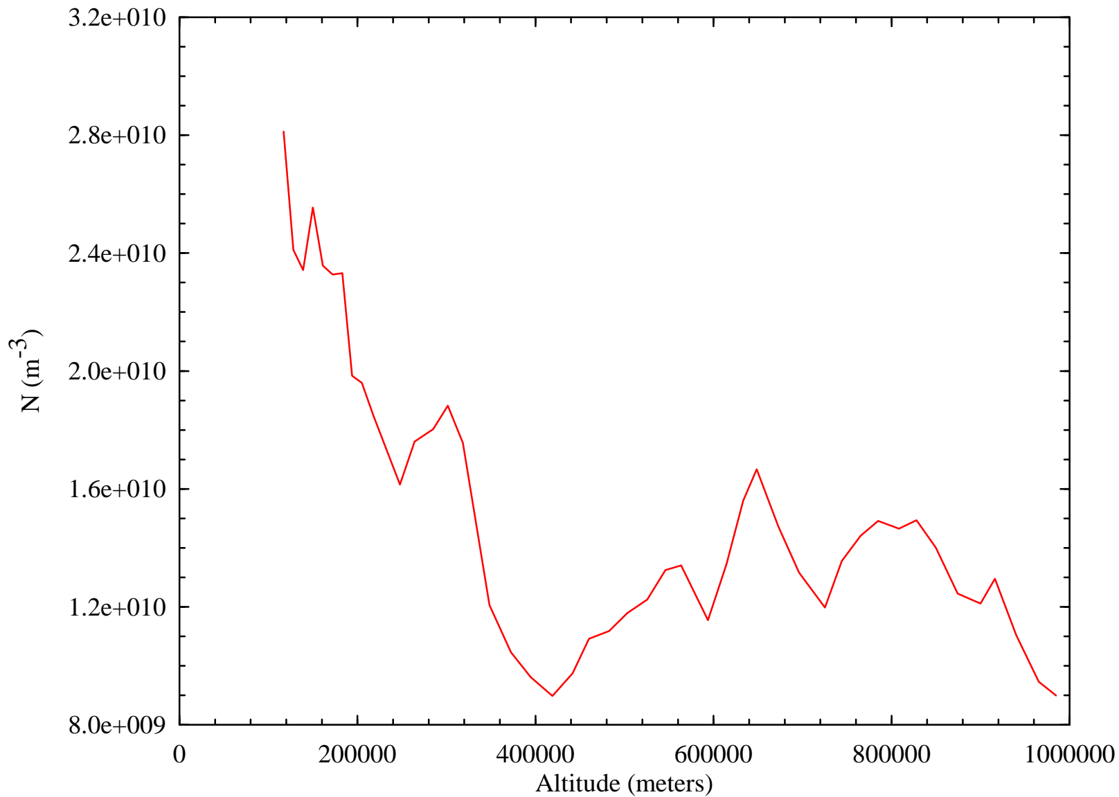
Electron Number Density vs. Altitude Derived from Io Radio Occultation (I09663NA)
