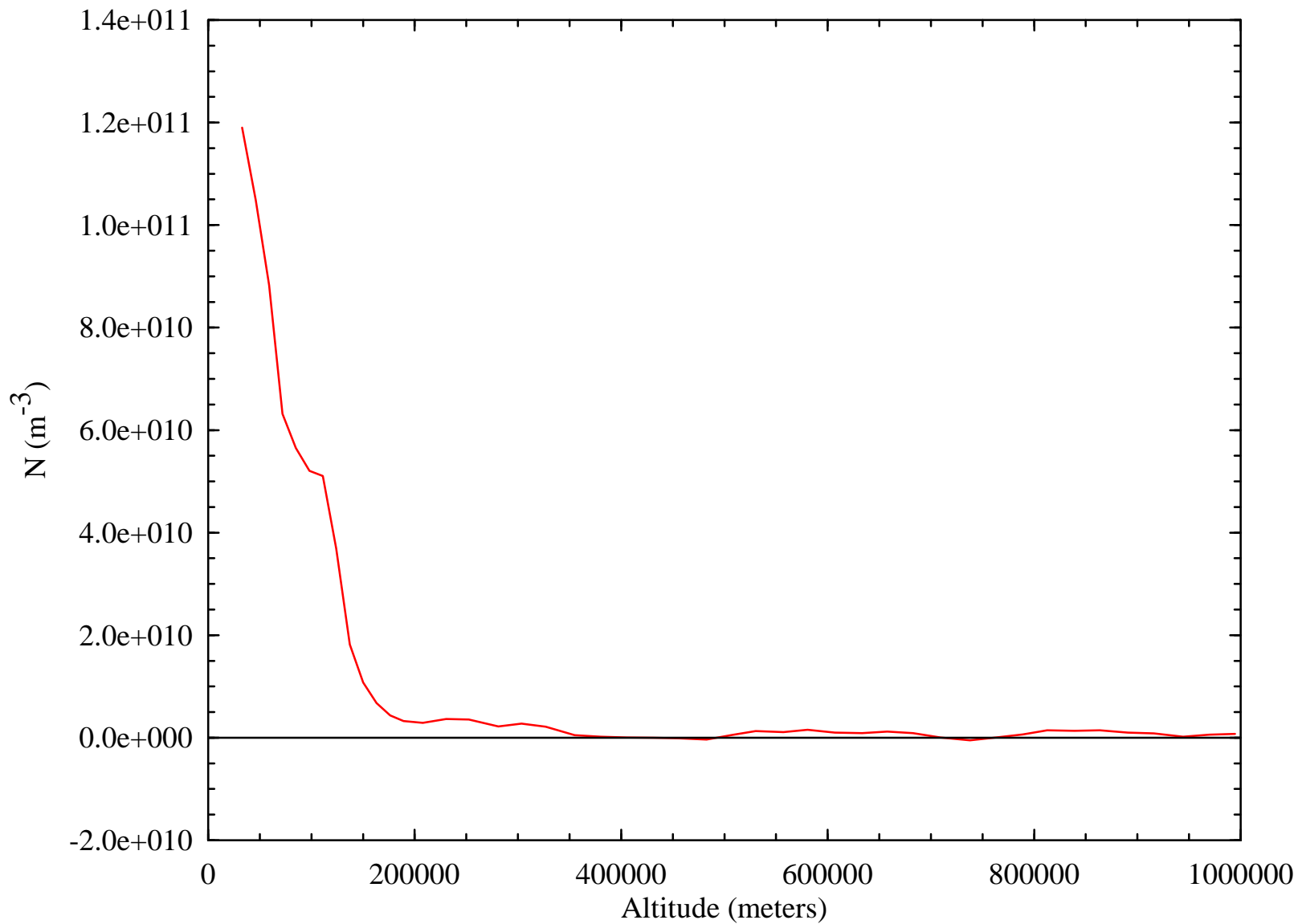
Electron Number Density vs. Altitude Derived from Io Radio Occultation (I09443XA)
