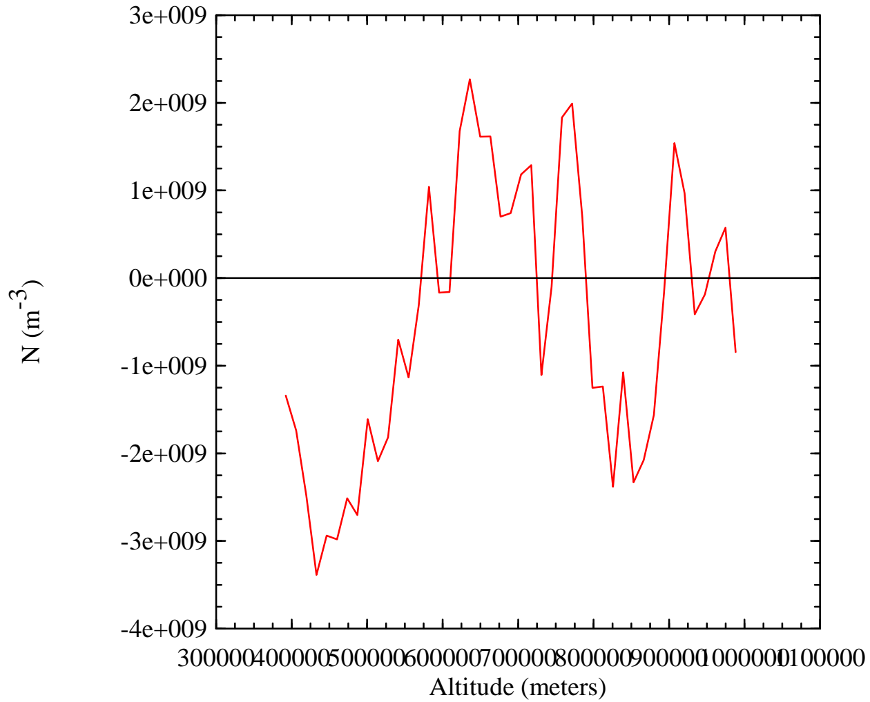
Electron Number Density vs. Altitude Derived from Io Radio Occultation (I09343XA)
