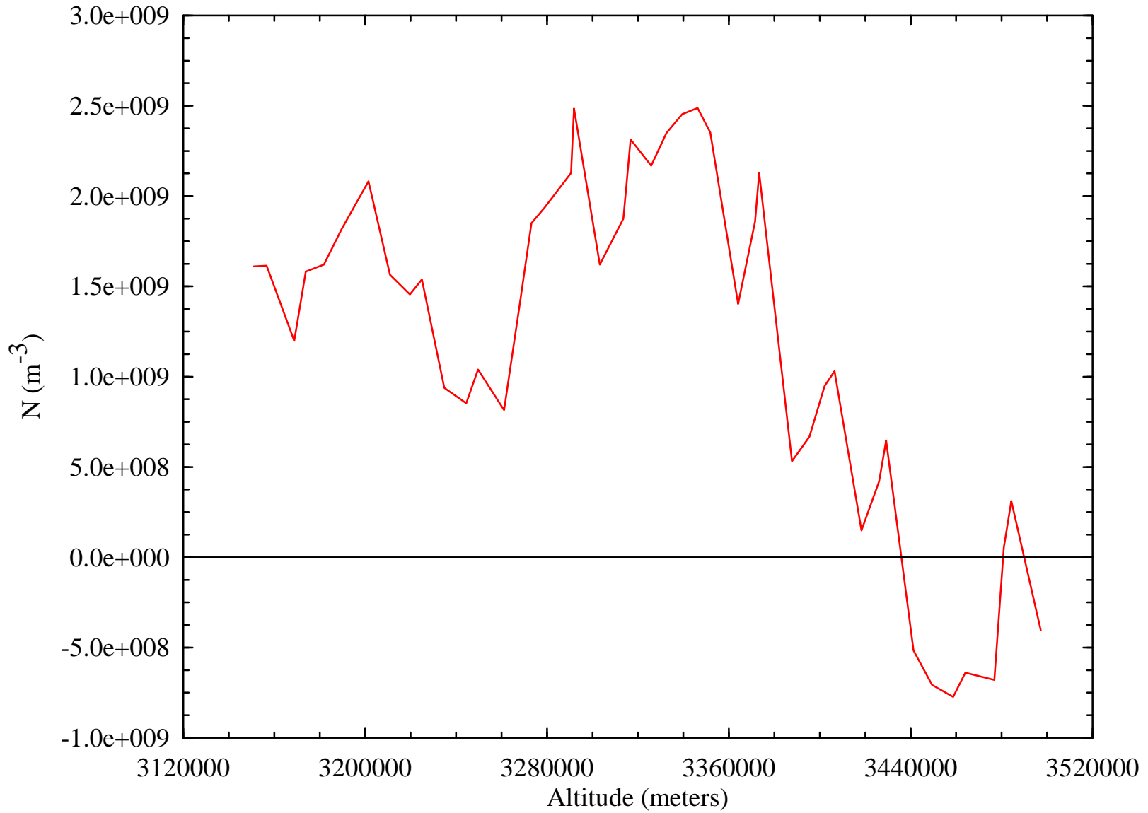
Electron Number Density vs. Altitude Derived from Jupiter Radio Occultation (J04_14NA)
